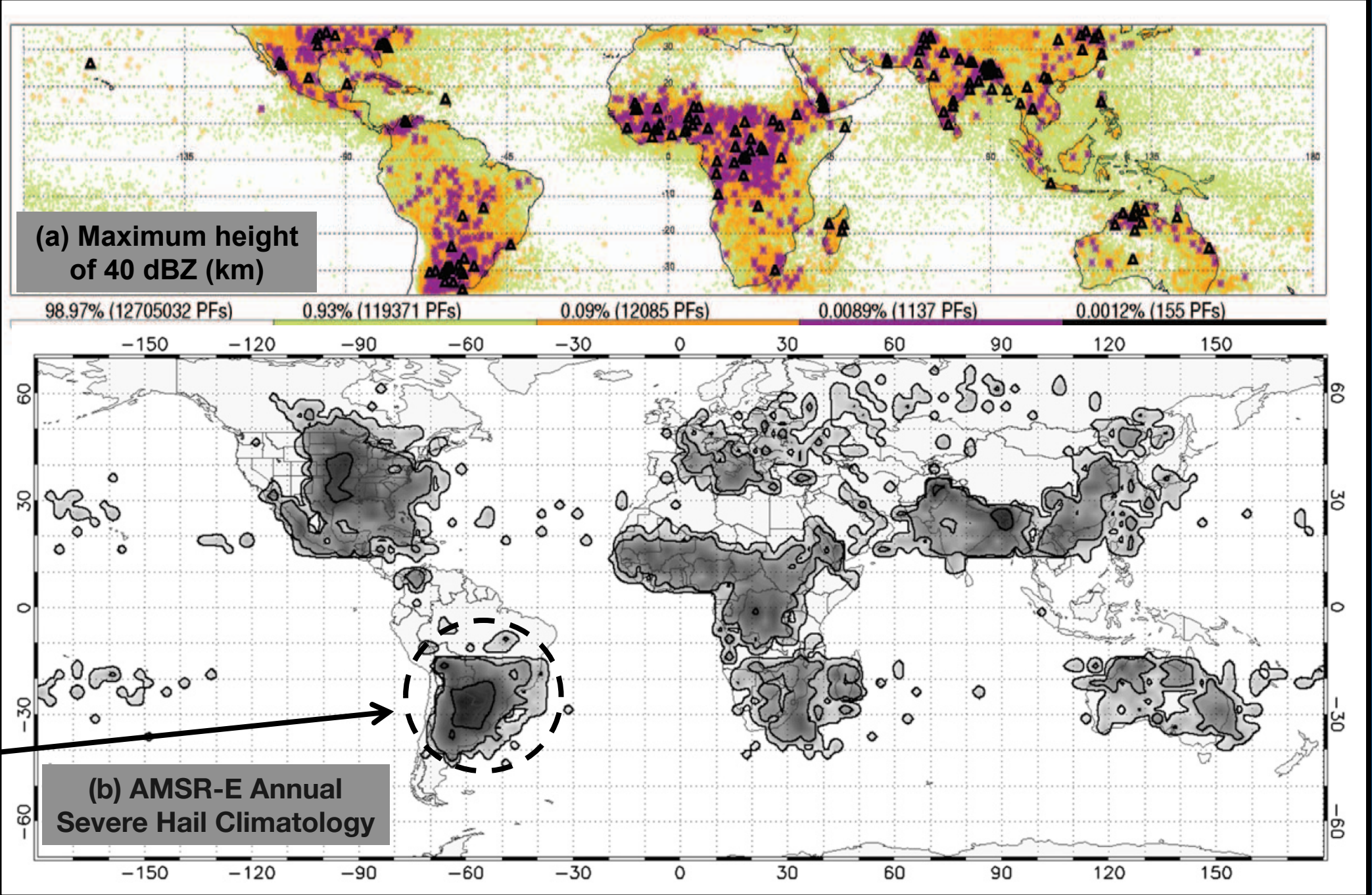
Figure 1. (a) Locations of intense convective events using the color code matching their rarity from Zipser et al. (2006). (b) AMSR-E annual severe hail (>1 in. diameter) climatology from Cecil and Blankenship (2012).
