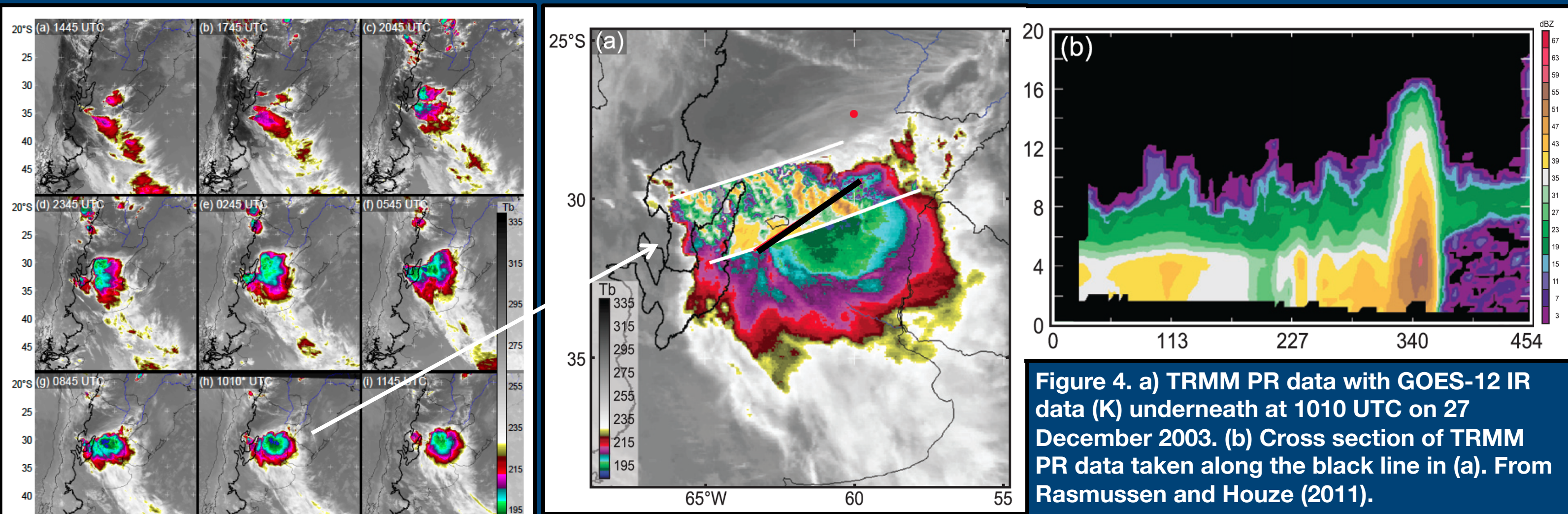
Figure 3. Sequence of infrared satellite images (K) showing storm initiation and evolution for the 26-27 December 2003 wide convective core. From Rasmussen and Houze (2011).
