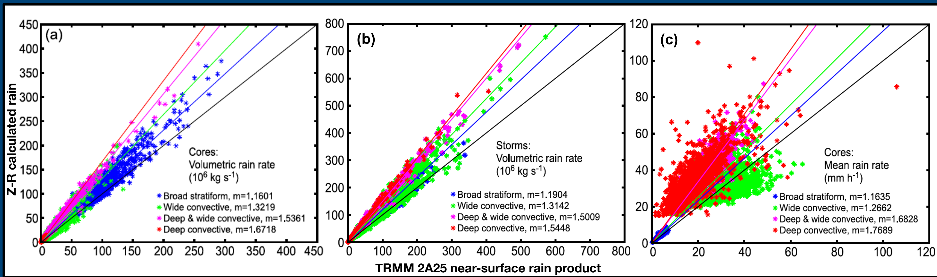
Figure 7. Volumetric and mean rain rates for various storm types in South America. (a) Volumetric rain rates from TRMM identified echo cores. (b) Volumetric rain rates from the full storm identified by TRMM that the echo cores are embedded within. (c) Mean rain rates from TRMM echo cores.
