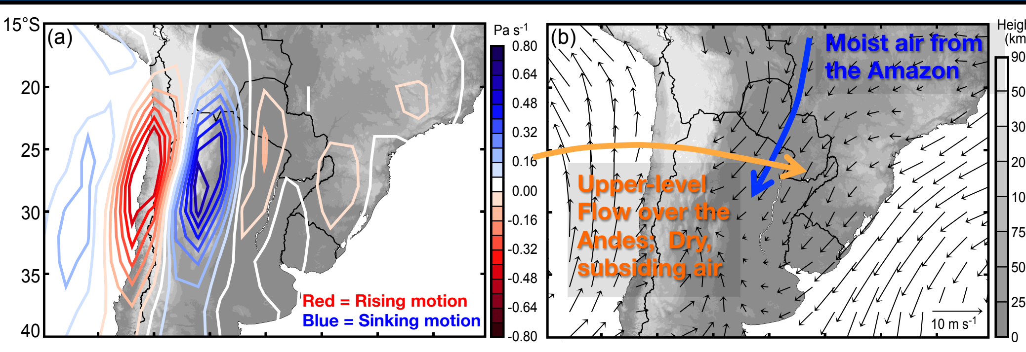
Figure 5. Climatological composite maps for days on which the TRMM PR showed storms containing wide convective cores over subtropical S. America. (a) Vertical motion (omega) and (b) 1000 mb winds. From Rasmussen and Houze (2011).
