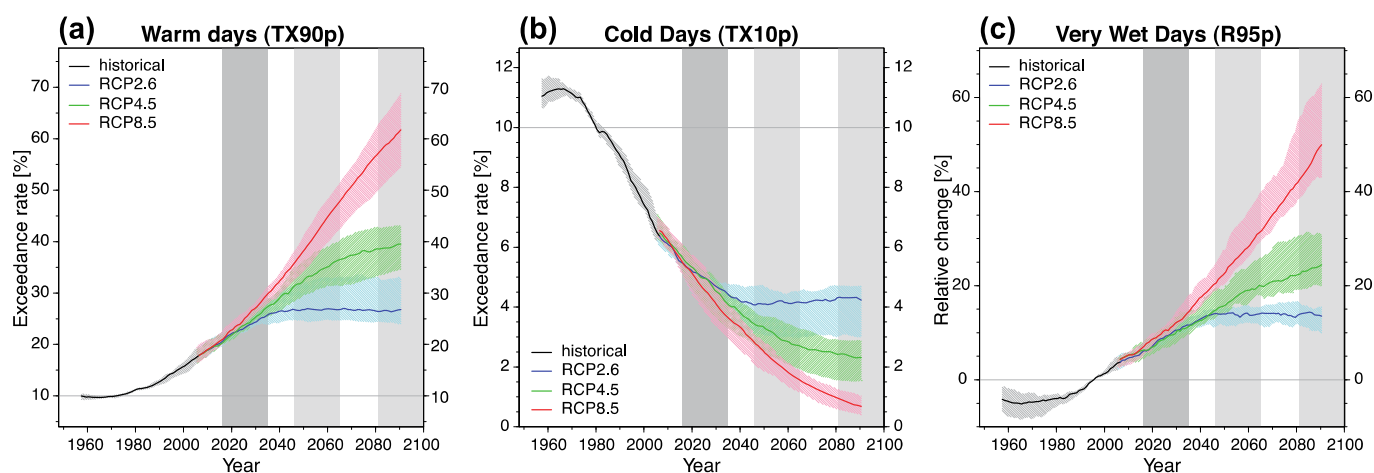
Figure 11.17: Global projections of the occurrence of (a) warm days (TX90p), (b) cold days (TX10p), and (c) precipitation amount from very wet days (R95p). Results are shown from CMIP5 for the RCP2.6, RCP4.5 and RCP8.5 scenarios. Solid lines indicate the ensemble median and shading indicates the interquartile spread between individual projections (25th and 75th percentiles). The specific definitions of the indices shown are (a) percentage of days annually with daily maximum surface air temperature ( T_{\max} ) exceeding the 90th percentile of T_{\max} for 1961–1990, (b) percentage of days with T_{\max} below the 10th percentile, and (c) percentage change relative to 1986–2005 of the annual precipitation amount from daily events above the 95th percentile. From Sillmann et al. (2013).
