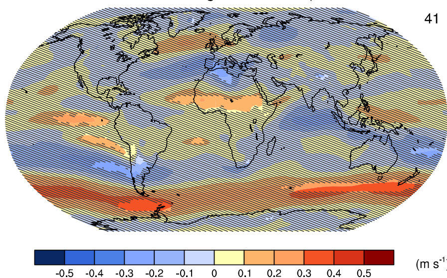
Figure 11.15: CMIP5 multi-model ensemble mean of projected changes [m/s] in zonal (west-to-east) wind at 850hPa for 2016–2035 relative to 1986–2005 under RCP4.5. The number of CMIP5 models used is indicated in the upper-right corner. Hatching and stippling as in Figure 11.10.
