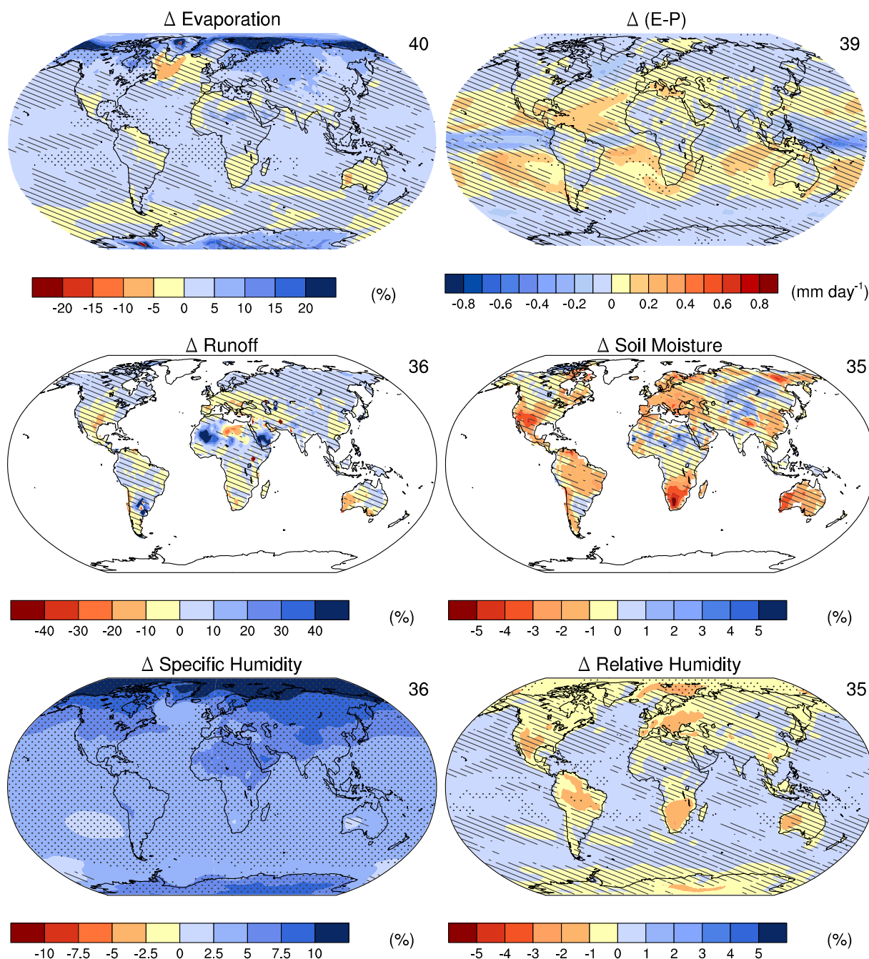
Figure 11.14: CMIP5 multi-model annual mean projected changes for the period 2016–2035 relative to 1986–2005 under RCP4.5 for: (a) evaporation (%), (b) evaporation minus precipitation (E-P, \text{mm day}^{-1} ), (c) total runoff (%), (d) soil moisture in the top 10 cm (%), (e) relative change in specific humidity (%), and (f) absolute change in relative humidity (%). The number of CMIP5 models used is indicated in the upper-right corner of each panel. Hatching and stippling as in Figure 11.10.
