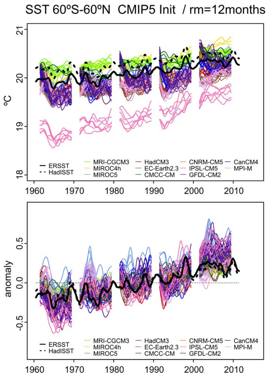
Figure 11.2: Time series of global-mean sea surface temperature from the a) direct model output and b) anomalies of the CMIP5 multi-model initialized hindcasts. Results for each forecast system are plotted with a different colour, with each line representing an individual member of the ensemble. Results for the start dates 1961, 1971, 1981, 1991 and 2001 are shown, while the model and observed climatologies to obtain the anomalies in panel b) have been estimated using data from start dates every five years. The reference data (ERSST) is drawn in black. All time series have been smoothed out with a 24-month centred moving average that filters out the seasonal cycle and removes data for the first and last years of each time series.
