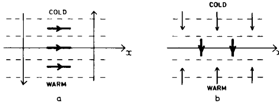
Figure 2. Illustration of the forcing terms when the potential temperature (dashed contours) is a function of y only with positive y pointing towards colder air. The motion is shown by light arrowed lines and Q by heavy arrowed lines. (a) Horizontal shear: v_\theta an increasing function of x only. Q_1 is positive and Q_2 zero (b) Confluence: v_\theta a decreasing function of y only. Q_1 is zero and Q_2 negative.
