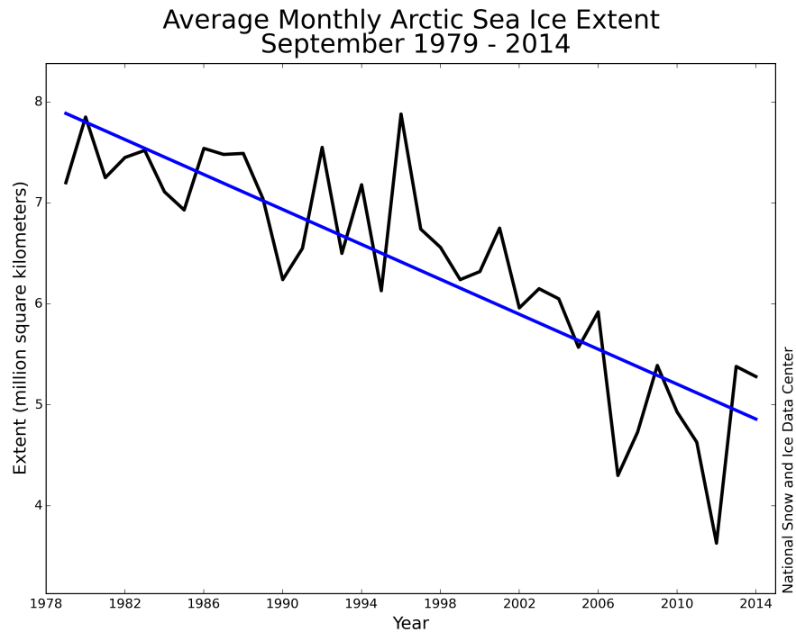
Figure 2. Arctic sea ice extent in September from 1979 to 2014. Data are from passive microwave satellite using the NASA team algorithm. Each of the lowest 10 years in this record occurred in the last decade. Figure downloaded from the National Snow Ice Data Center, retrieved 2 March 2015 from http://nsidc.org/arcticseaicenews/2014/10/ .
