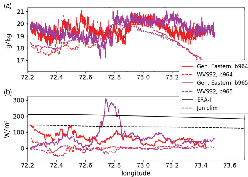
FIGURE 13 (a) Specific humidity ( \text{g/kg} ) and (b) estimates of surface latent heat flux ( \text{W/m}^2 ) from low-level runs over the Arabian Sea (colours), ERA-Interim on 26 June, 0000–1200 UTC mean (solid black, 0530 to 1730 local time), and Goddard Satellite-based Surface Turbulent Fluxes (GSSTF, dashed black) climatology for June 1998–2008 [Colour figure can be viewed at wileyonlinelibrary.com ]
