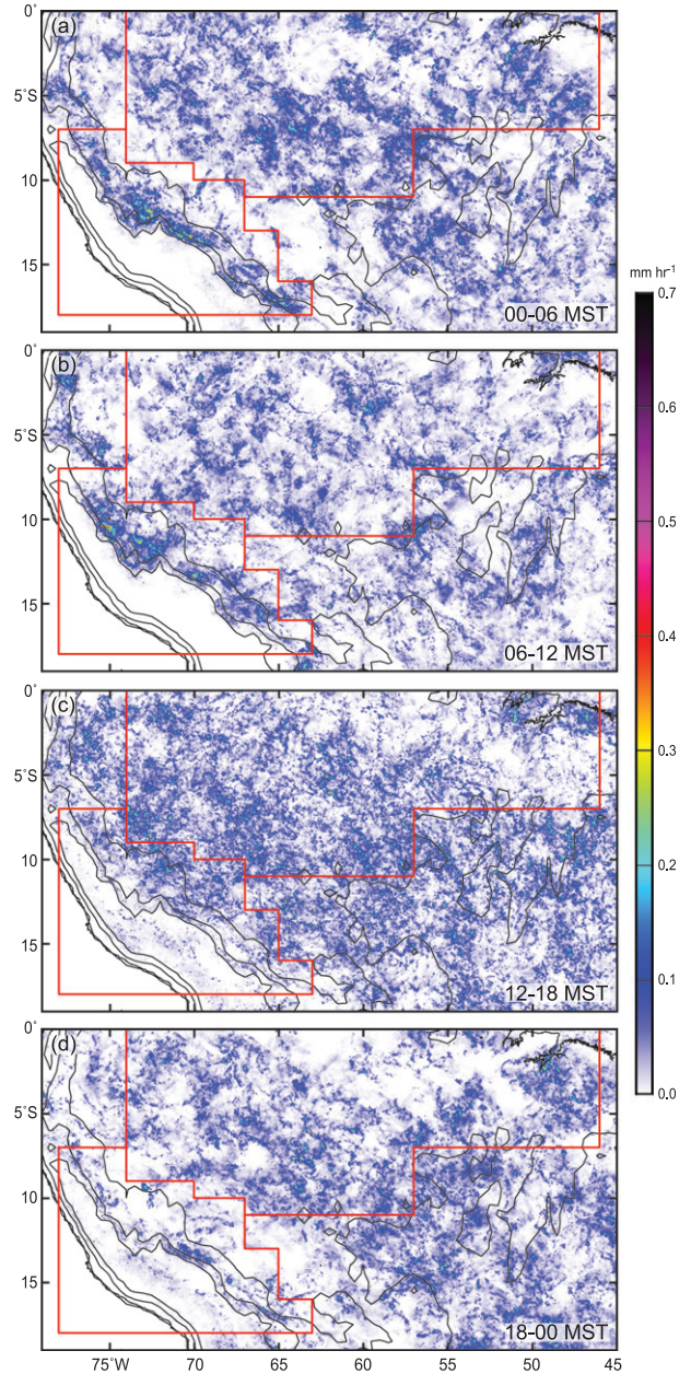
FIG. 12. As in Fig. 7 but for medium systems in the continental tropics.
