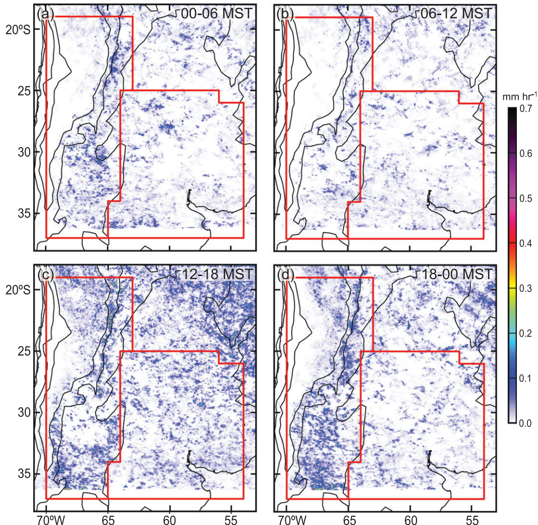
FIG. 7. Precipitation from small systems occurring (a) between 0000 and 0600 MST, (b) between 0600 and 1200 MST, (c) between 1200 and 1800 MST, and (d) between 1800 and 0000 MST in the continental subtropics. Orographic contours as in Fig. 2; the outlined regions are defined in Fig. 1.
