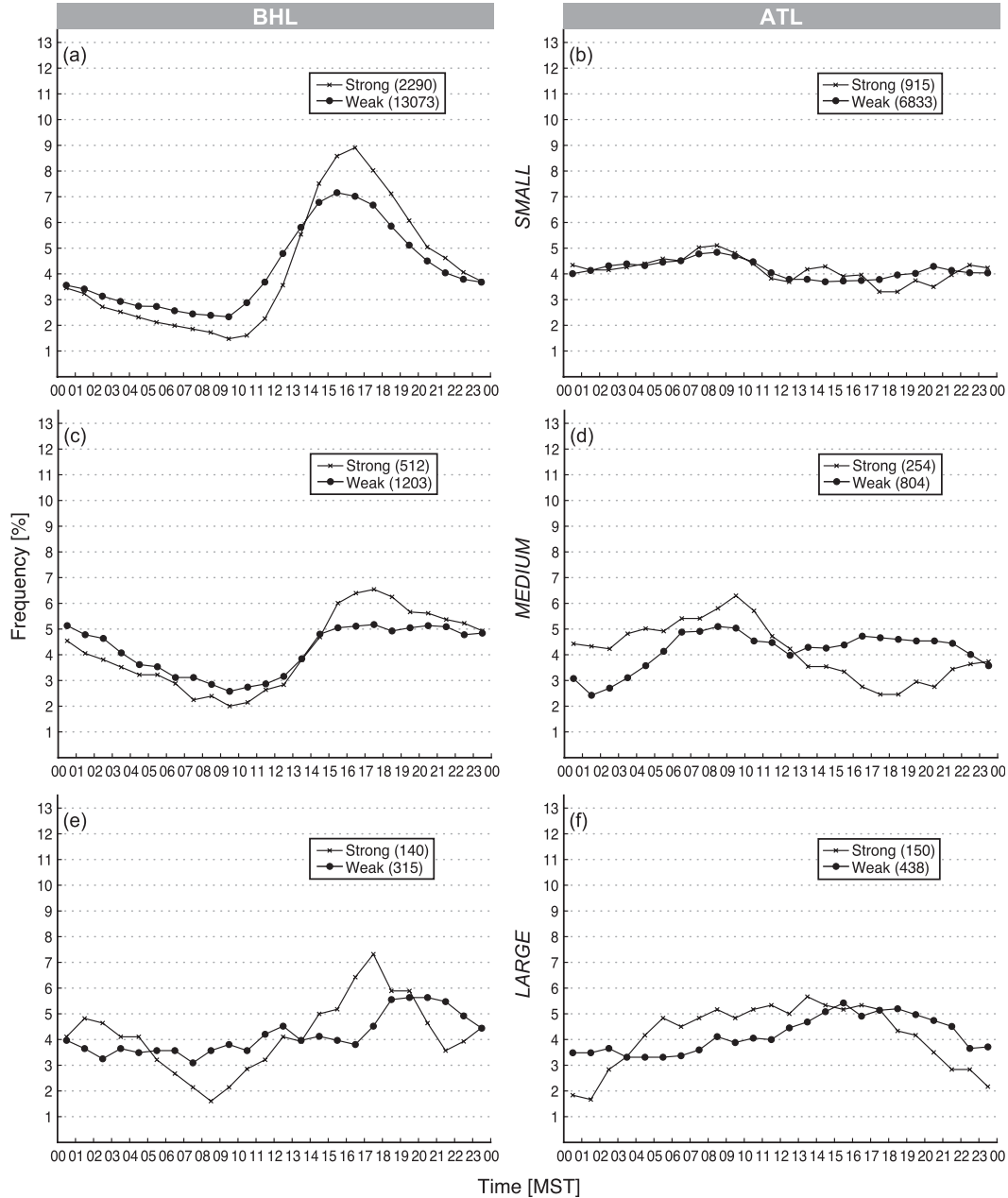
FIG. 14. As in Fig. 6 but for systems in the BHL and ATL regions.
