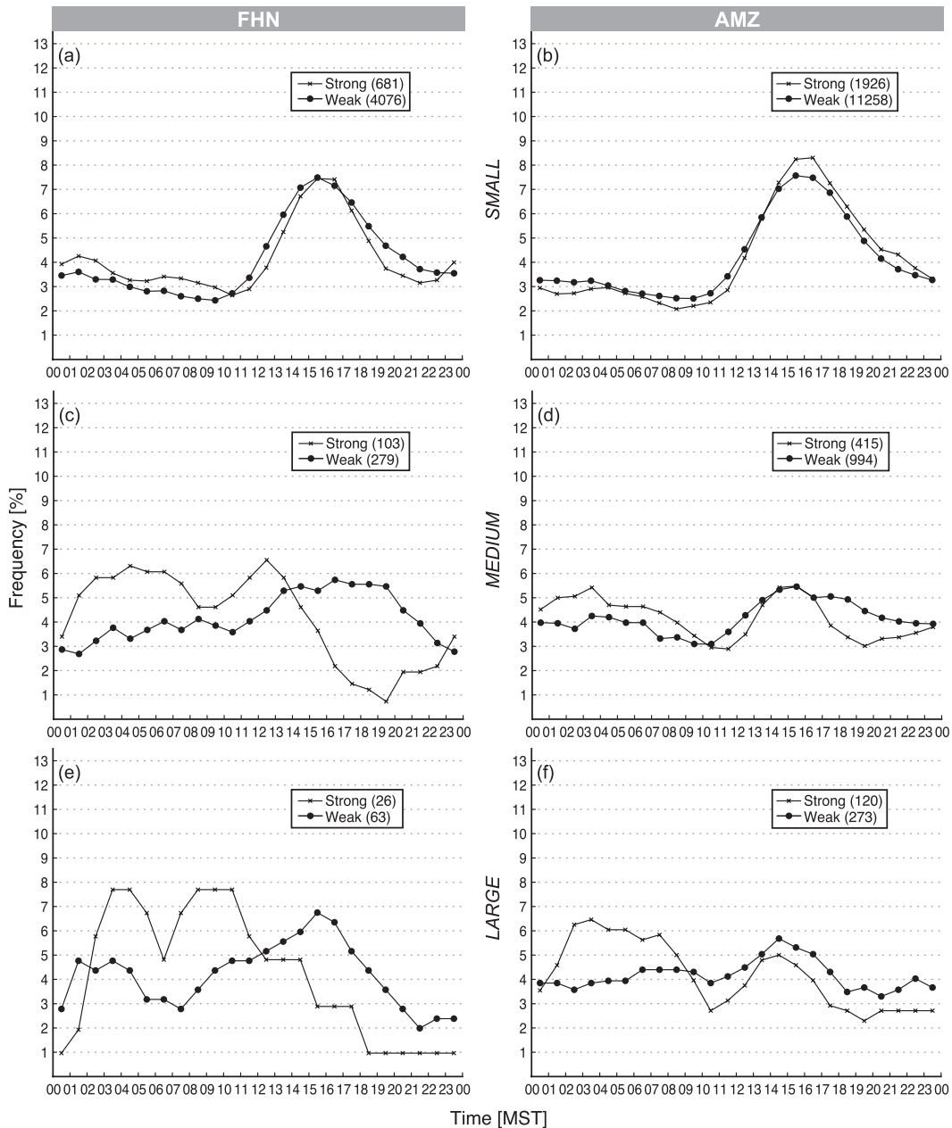
FIG. 10. As in Fig. 6 but for echoes in the FHN and AMZ regions.
