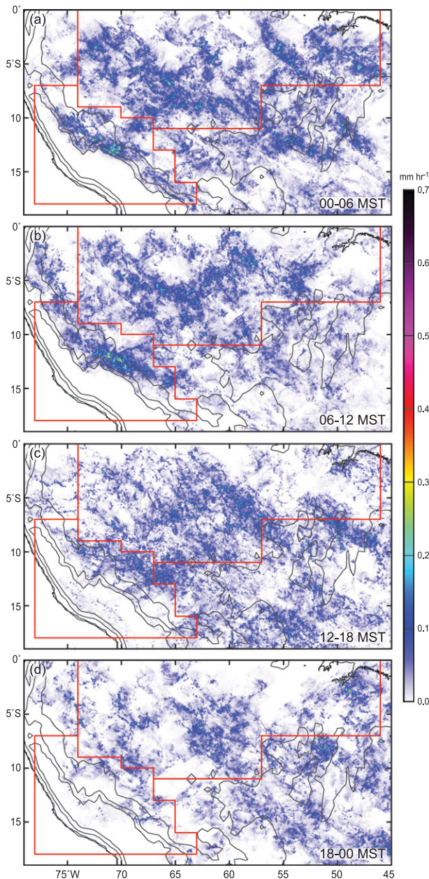
FIG. 13. As in Fig. 7 but for large systems in the continental tropics.
