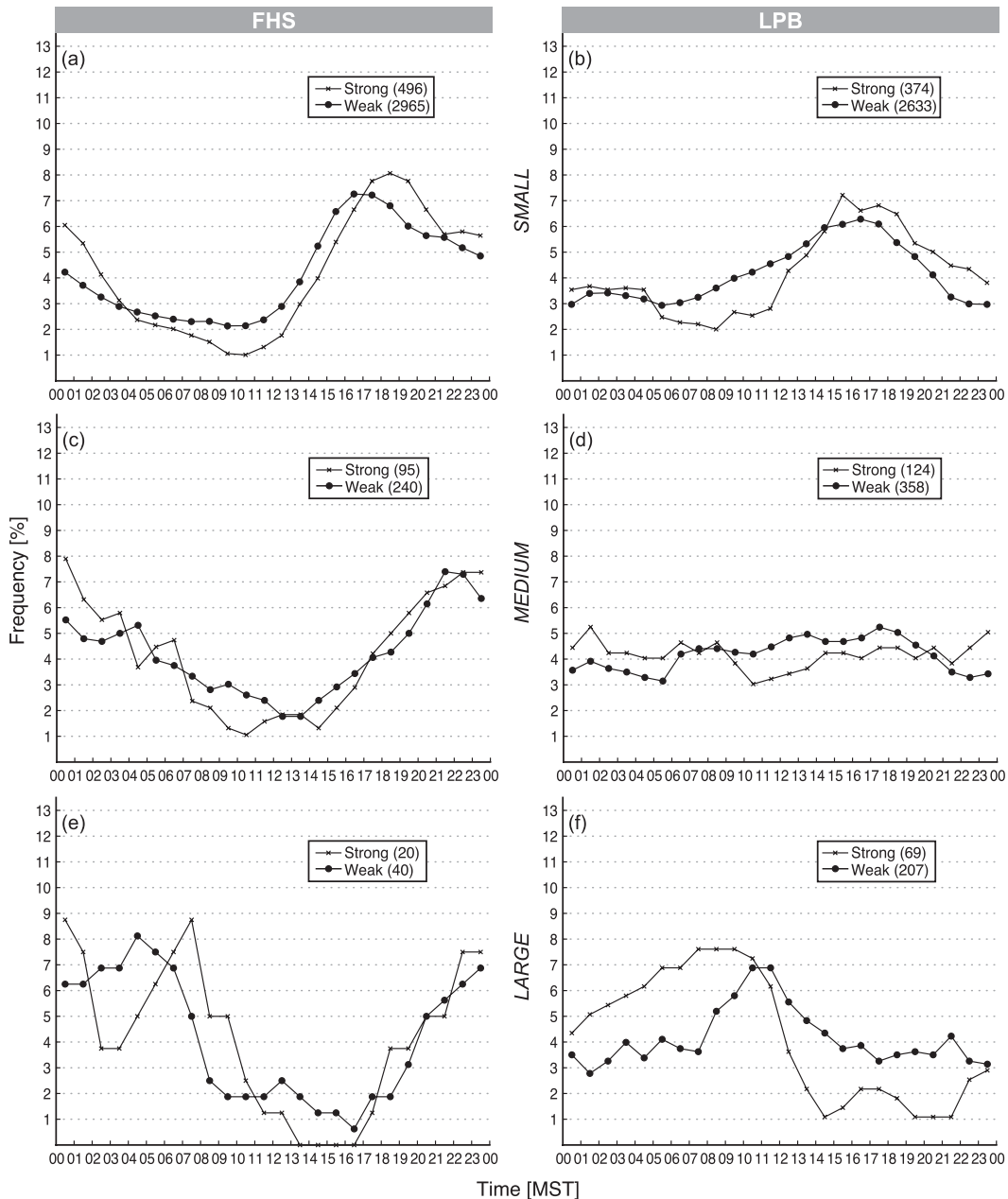
FIG. 6. Diurnal cycles of strong and weak small, medium, and large echoes in the FHS and LPB regions.
