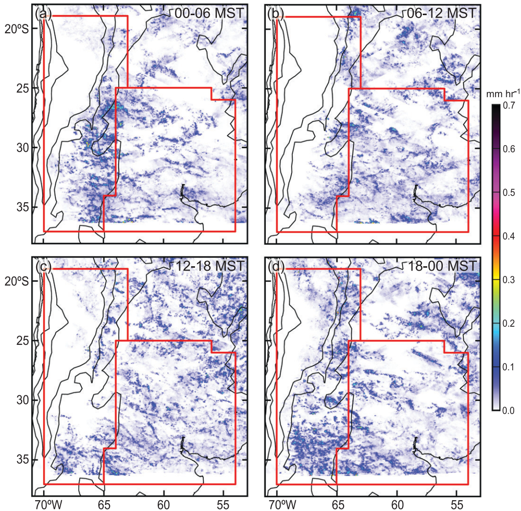
FIG. 8. As in Fig. 7 but for medium echoes.
