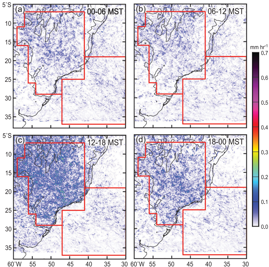
FIG. 15. As in Fig. 7 but for small systems in the SACZ.
