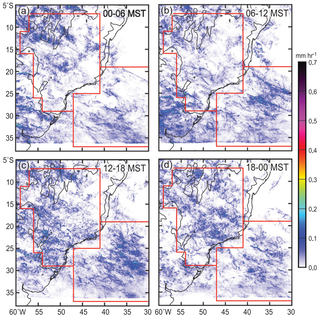
FIG. 17. As in Fig. 7 but for large systems in the SACZ.
