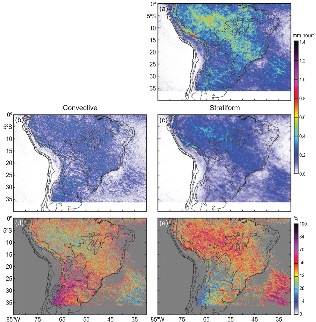
FIG. 2. Summer precipitation means of (a) total rain, (b) convective rain, (c) stratiform rain, (d) convective percentage, and (e) stratiform percentage. Pixels where the total precipitation is < 0.15 \text{ mm h}^{-1} are deleted. Topographic contours of 0.3 km, 1.5 km, and 3 km are shown in black.
