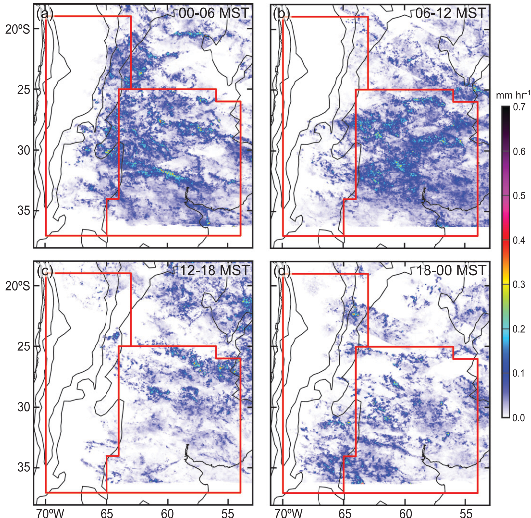
FIG. 9. As in Fig. 7 but for large echoes.
