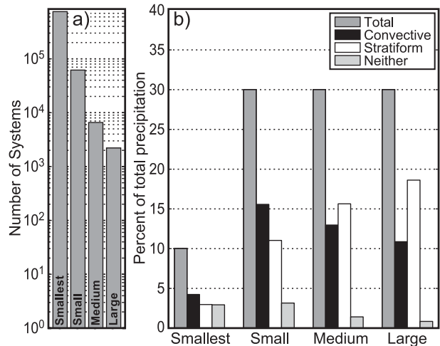
FIG. 3. (a) Total number of echo objects in the four size categories defined in the text. (b) Percentage that each type of system contributes to the total precipitation.
