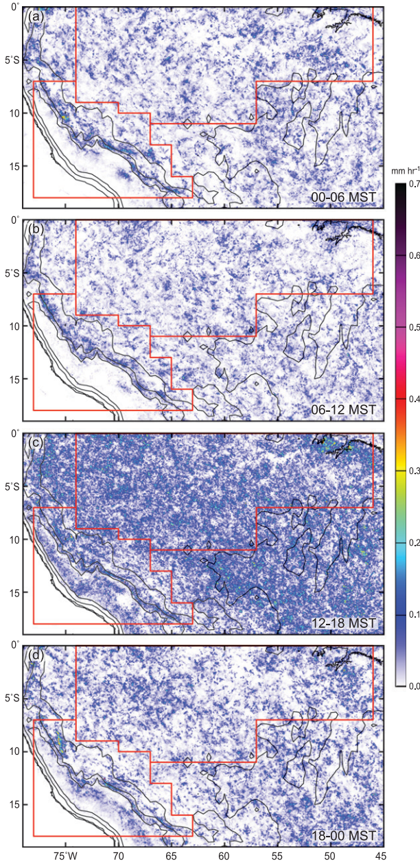
FIG. 11. As in Fig. 7 but for the continental tropics.
