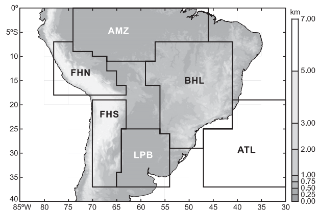
FIG. 1. Topography of the region of interest and subregions: La Plata basin (LPB), western South Atlantic (ATL), Brazilian Highlands (BHL), Amazon basin (AMZ), northeastern and southeastern foothills of the Central Andes (FHN and FHS, respectively). Higher topography is in lighter shading.
