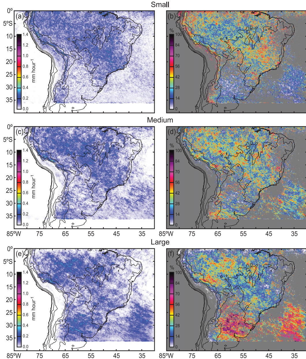
FIG. 4. Precipitation patterns from small, medium, and large echoes: (left) total rain and (right) percentage. Orographic contours as in Fig. 2.
