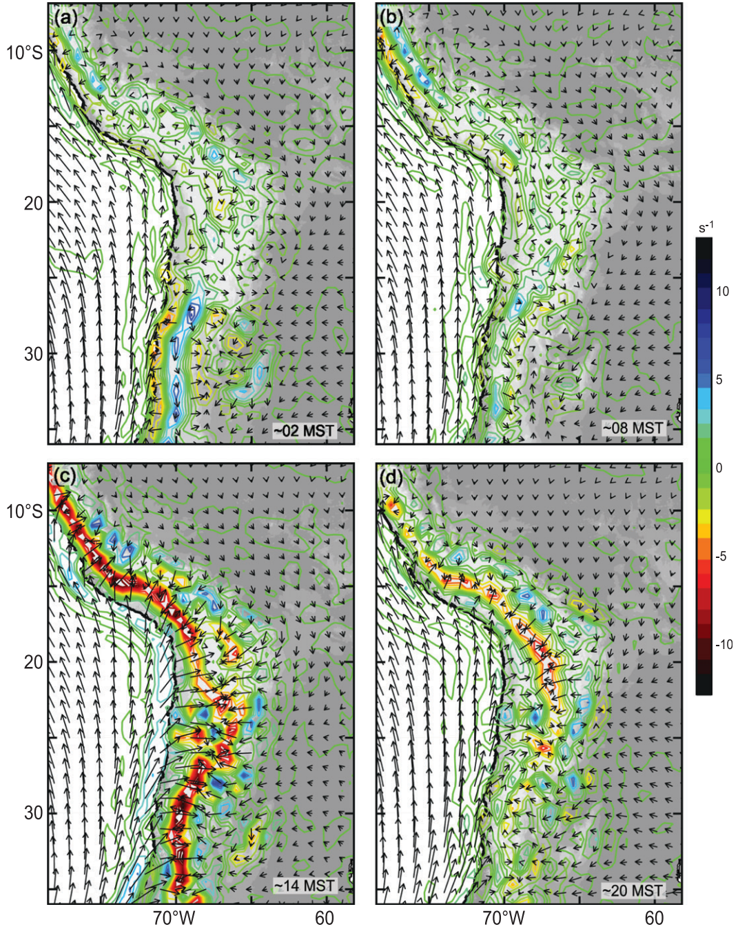
FIG. 5. NCEP CFSR 10-m winds ( \text{m s}^{-1} ) and divergence ( \text{s}^{-1} ) climatology at (a) 0600 UTC ( \sim 0200 MST), (b) 1200 UTC ( \sim 0800 MST), (c) 1800 UTC ( \sim 1400 MST), and (d) 0000 UTC ( \sim 2000 MST), MST \equiv mean solar (local) time. For better readability the wind vectors are shown at 1^\circ resolution.
