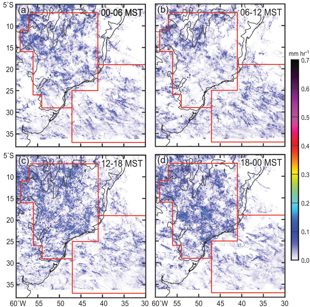
FIG. 16. As in Fig. 7 but for medium systems in the SACZ.
