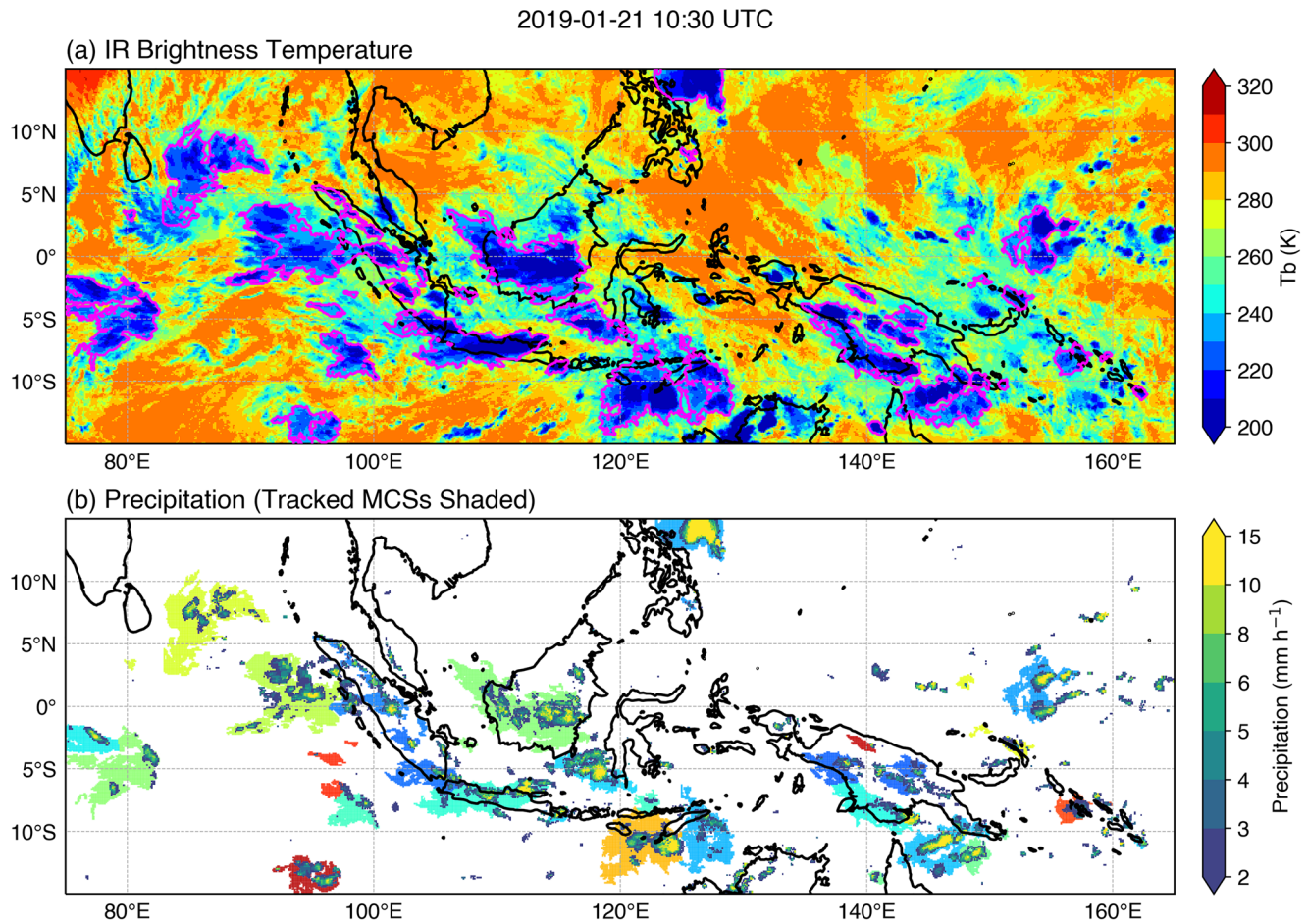
Figure 7. Example snapshot of tracked MCSs over the Maritime Continent at 10:30 UTC on January 21, 2019. (a) Infrared brightness temperature, (b) GPM IMERG precipitation. The magenta contours in (a) and the color shadings behind large clusters of PFs in (b) denote each tracked MCS. Weak rain rates <2 \text{ mm h}^{-1} in (b) are excluded for clarity. Animation for this day is provided in the Supporting Information. GPM, Global Precipitation Measurement; IMERG, Integrated Multi-satellite Retrievals for GPM; MCS, mesoscale convective system; PF, precipitation feature.
