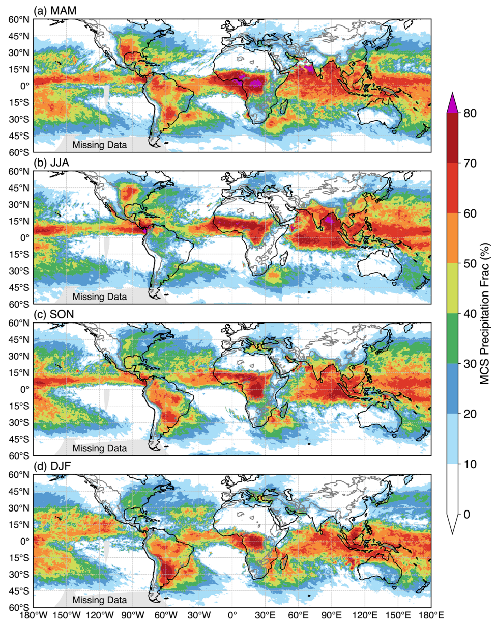
Figure 11. Percentage of MCS precipitation to total precipitation in (a) March–May, (b) June–August, (c) September–November, and (d) December–February. MCS, mesoscale convective system.
