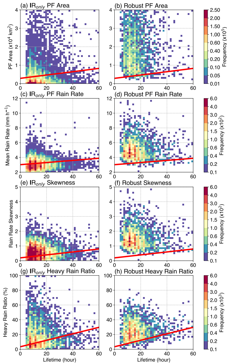
Figure 9. Comparisons of the joint PDF of PF parameters between MCSs defined by the IR-only method (left column) and the new IR + PF method (right column) over Central Asia region (28°N–60°N, 50°E–120°E) for all seasons during 2014–2019. (a, b) PF area, (c, d) PF mean rain rate, (e, f), PF rain rate skewness, and (g, h) heavy rain ratio. Red lines denote thresholds used to define robust MCSs for each PF parameter. The MCS lifetime here is defined by the tracked CCS duration. Mean values of the PF parameters throughout each MCS lifetime are used. IR, infrared; MCS, mesoscale convective system; PDF, probability density function; PF, precipitation feature.
