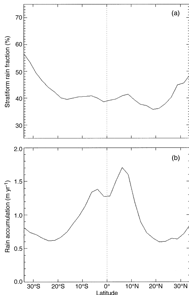
FIG. 2. The PR 2.5° zonal averages at near surface from 1998 to 2000 for (a) stratiform rain fraction and (b) rain accumulation.
