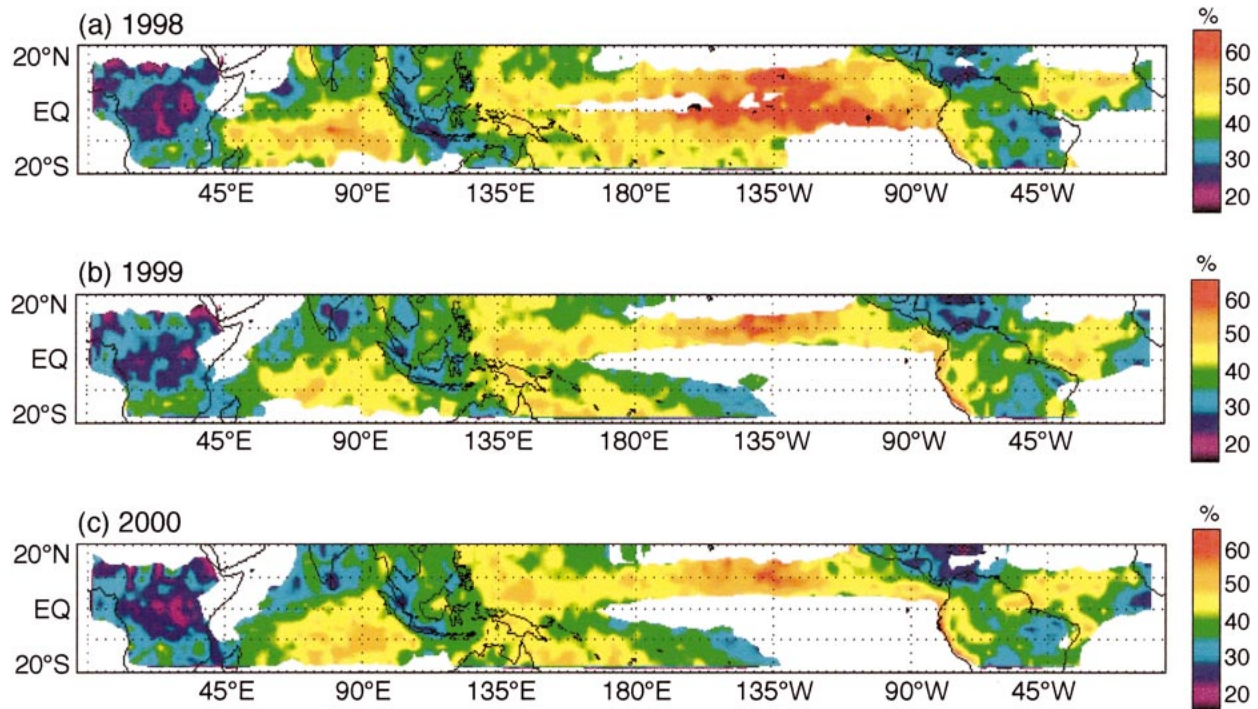
FIG. 8. Annual averages of PR stratiform rain fraction based on 2.5^\circ grid averages for 1998, 1999, and 2000. Areas with annually averaged rain of less than 0.6 \text{ m yr}^{-1} were not included.
