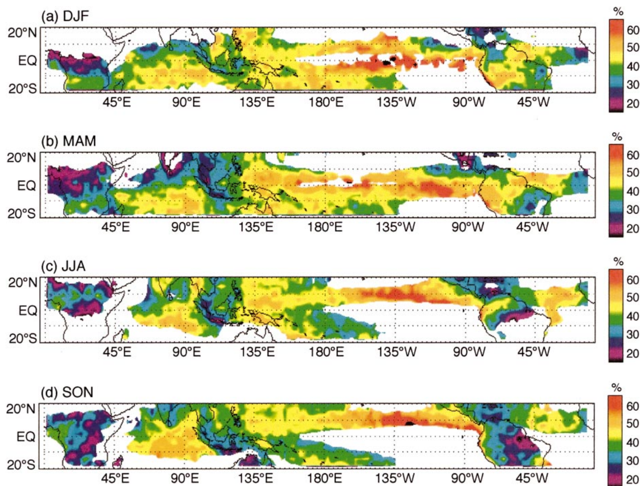
FIG. 7. Seasonal PR stratiform rain fraction based on 2.5^\circ grid averages for 1998–2000. Areas with annually averaged rain of less than 0.6 \text{ m yr}^{-1} were not included.
