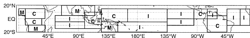
FIG. 10. Quasi-steady circulation regions defined as I (intertropical convergence zone), M (seasonal monsoon regions), and C (semipermanent equatorial convective zones).
