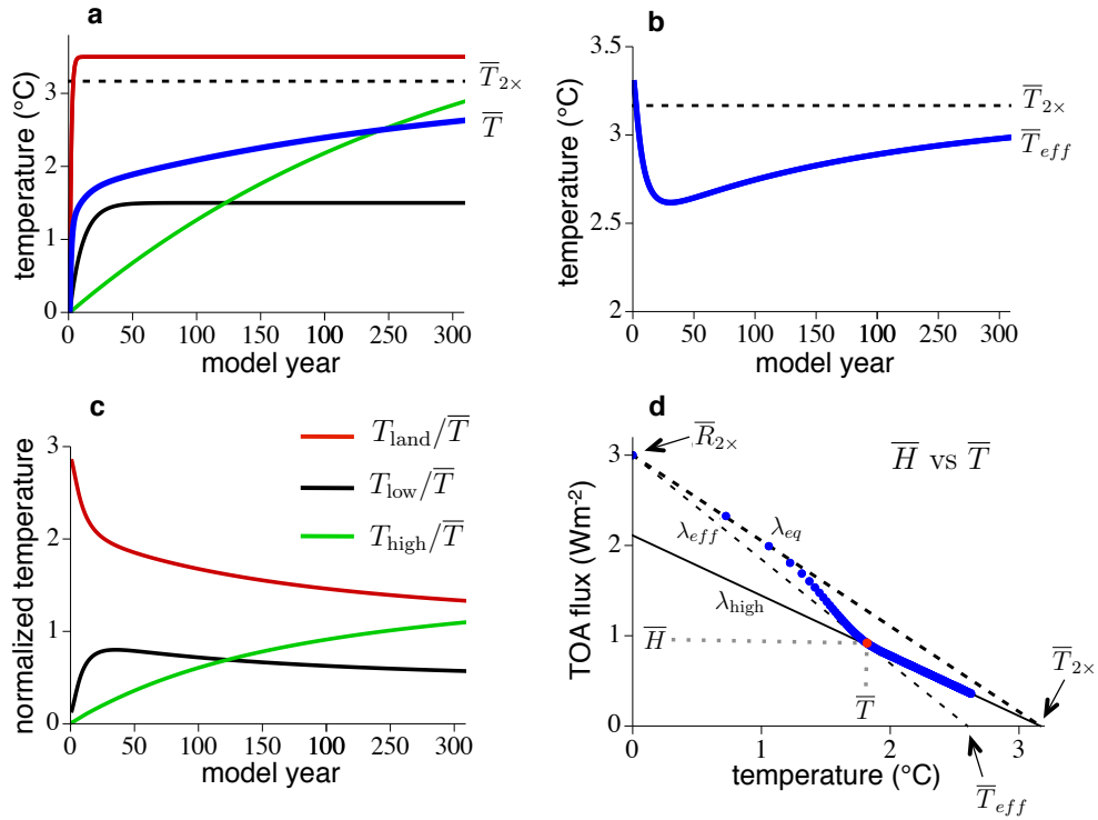
FIG. 6. Temperature and effective climate sensitivity in a three-region energy balance climate model. a , Global mean (blue), land (red), low-latitude ocean (black) and high-latitude ocean (green) surface temperature change following an abrupt doubling of \text{CO}_2 in year zero, b , effective climate sensitivity, c , regional temperature change normalized by global mean temperature change, and d , global TOA energy flux plotted against global mean temperature change. The red dot indicates a particular year with global energy flux equal to \bar{H} and global-mean temperature equal to \bar{T} . \bar{T}_{eff} at this time can be schematically represented as the extrapolation of the thin dashed line (with slope \lambda_{eff} ) from point [0, \bar{R}_{2\times}] through this dot to the \bar{T} -axis. Late in the simulation, \bar{T}_{2\times} can be estimated by extrapolating a regression line (solid line with slope \lambda_{high} ) to the \bar{T} -axis. The thick dashed line (with slope \lambda_{eq} ) connecting points [0, \bar{R}_{2\times}] and [\bar{T}_{2\times}, 0] is the expected trajectory of points under the assumption that T_{eff} is constant.
