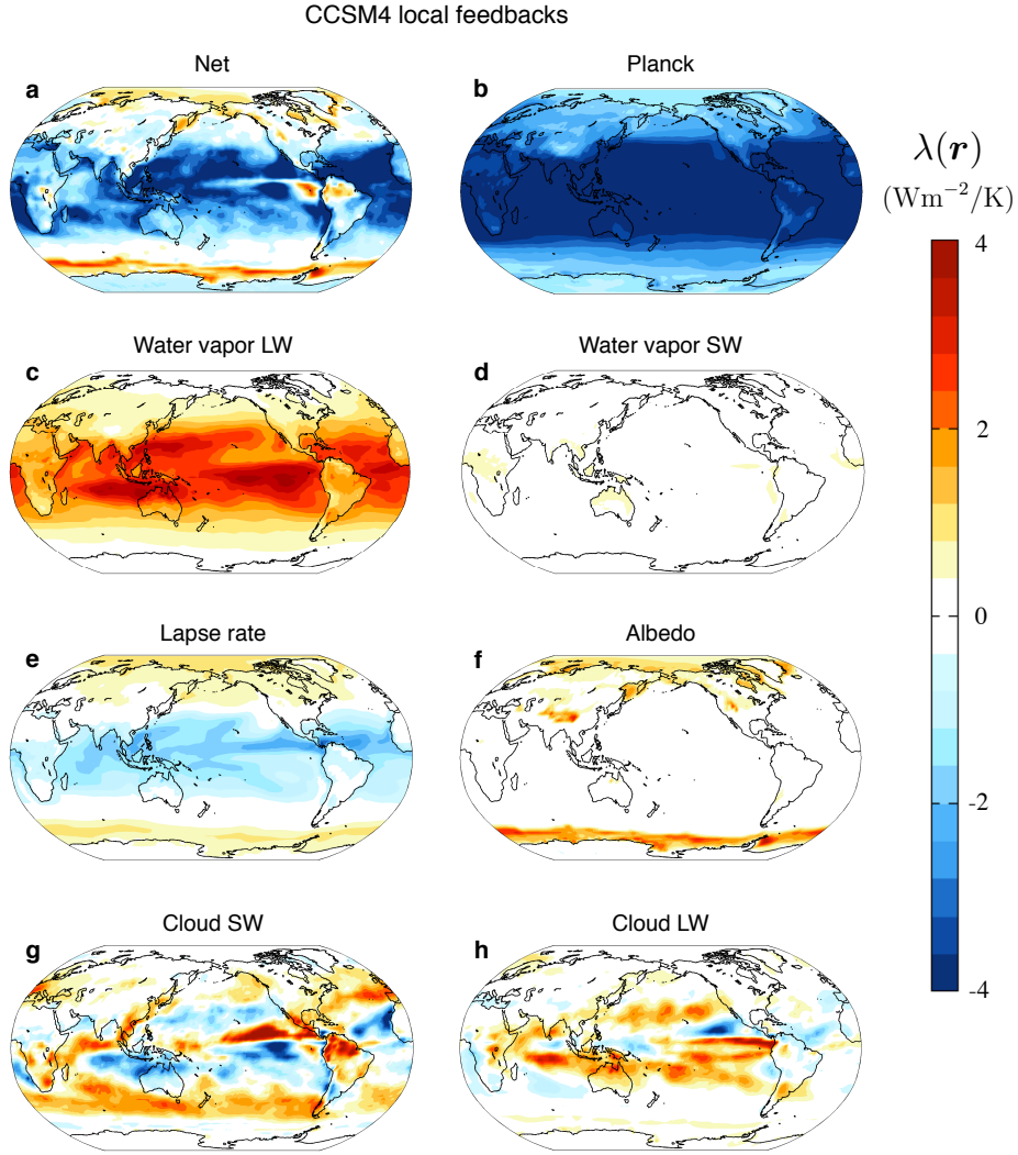
FIG. 5. Spatial patterns of net and individual local feedbacks within CCSM4. Local feedbacks (local TOA response per degree local surface temperature change), separated into a , Net (sum of all individual feedbacks), b , Planck, c , LW water vapor, d , SW water vapor, e , lapse rate, f , surface albedo, g , SW cloud, and h , LW cloud feedbacks.
