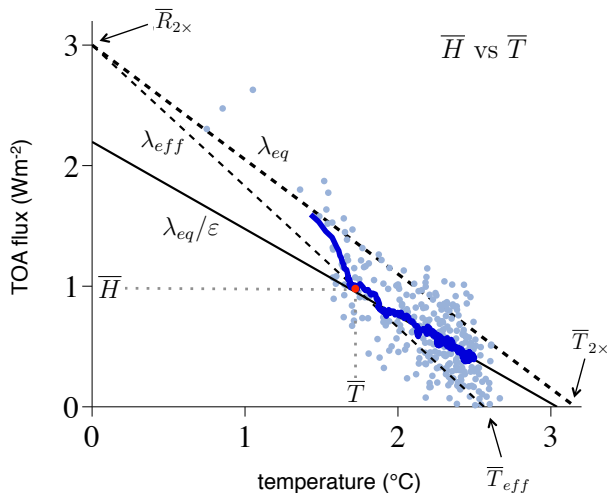
FIG. 7. CCSM4 TOA energy flux plotted against global annual mean temperature change. Light blue dots show individual years, and the dark blue line shows the 20-year running mean. The red dot indicates a particular decade with global energy flux equal to \bar{H} and global-mean temperature equal to \bar{T} . \bar{T}_{eff} at this time can be schematically represented as the extrapolation of the thin dashed line (with slope \lambda_{eff} ) from point [0, \bar{R}_{2\times}] through this dot to the \bar{T} -axis. Late in the simulation, \bar{T}_{2\times} can be estimated by extrapolating a regression line (solid line with slope \lambda_{eq}/\varepsilon ) to the \bar{T} -axis. The regression is performed over the final two centuries of the simulation.
