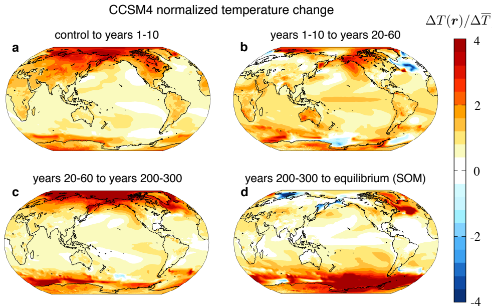
FIG. 3. Spatial patterns of warming within CCSM4. Regional surface temperature change normalized by global mean surface temperature change between the periods a , ‘control’ to years 1-10, b , years 1-10 to 20-60, c , years 20-60 to 200-300, and d , years 200-300 to equilibrium (as estimated by the SOM).
