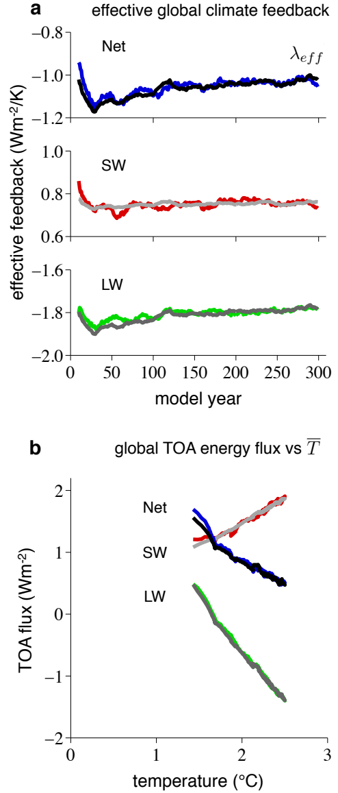
FIG. 2. Evolution of effective climate feedbacks and TOA energy flux within CCSM4. a , Net, SW and LW effective climate feedbacks, diagnosed from global energy balance (Eq. (2); blue, red, and green, respectively) and calculated with regional feedbacks (Eq. (8); black, light gray, and dark gray, respectively) and b , Global net, SW and LW TOA radiation flux as a function of global annual mean surface temperature change from the simulation (blue, red and green respectively) and as predicted from Eq. (2) using the calculated effective feedbacks (black, light gray, and dark gray, respectively). See Appendix A for the CO 2 radiative forcing employed here. All lines show 20-year running means.
