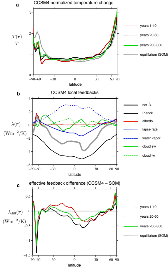
FIG. 4. Zonal-mean warming and local feedbacks within CCSM4. a , Regional surface temperature change normalized by global mean surface temperature change, b , Local net feedback (grey) and individual feedbacks, as in Fig. 5; the individual feedbacks everywhere sum to the net feedback \lambda(\mathbf{r}) , and c , Effective feedback from CCSM4 minus effective feedback from the SOM; the area-weighted global mean of each curve is equal to \lambda_{eff} - \lambda_{eq} .
