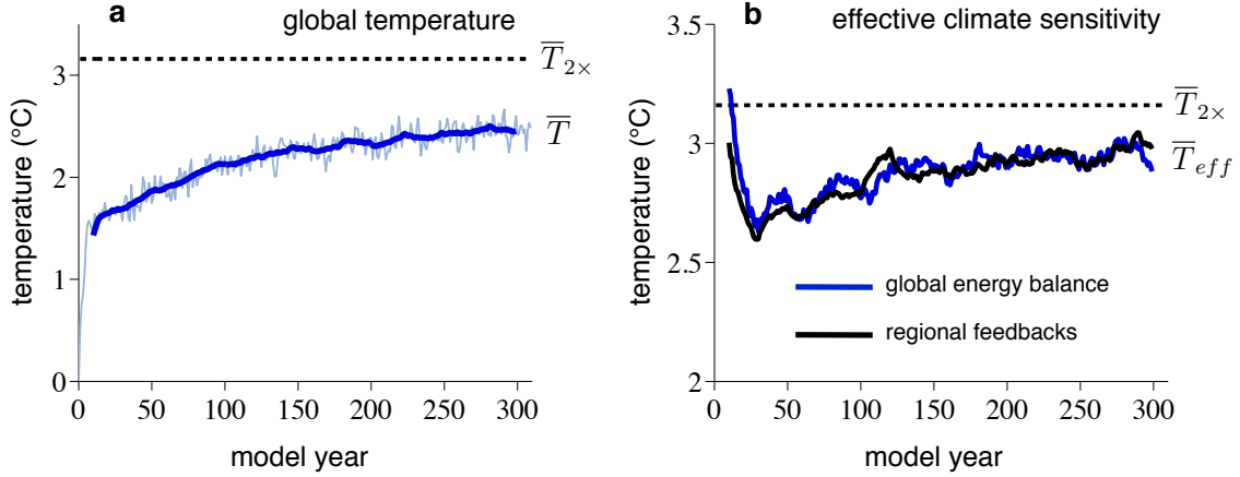
FIG. 1. Evolution of global temperature and effective climate sensitivity within CCSM4. a , Global annual mean surface temperature change \bar{T} , and b , effective climate sensitivity \bar{T}_{eff} within CCSM4 following an abrupt doubling of atmospheric \text{CO}_2 in year zero. \bar{T}_{eff} diagnosed by global energy balance (Eq. (4)) is shown in blue, and \bar{T}_{eff} calculated with regional feedbacks (Eq. (8)) is shown in black. Thick lines show 20-year running means. Equilibrium climate sensitivity \bar{T}_{2\times} is estimated from a slab ocean version of the model.
