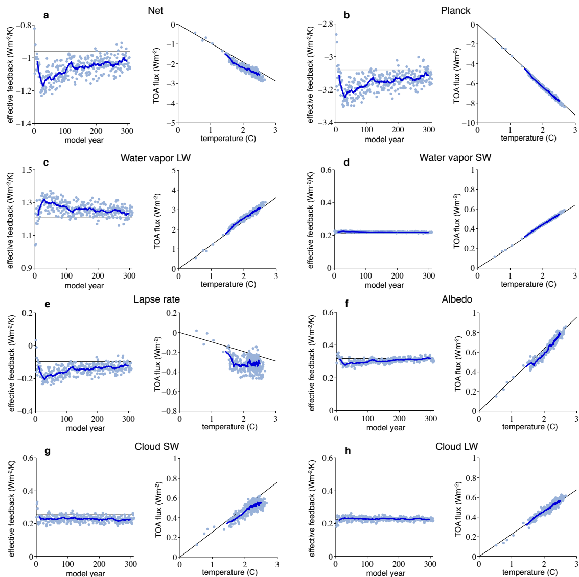
FIG. 8. Evolution of individual global effective climate feedbacks and associated TOA energy flux. Global effective climate feedbacks calculated with regional feedbacks (Eq. (8)), and associated global TOA energy flux as a function of global annual mean surface temperature change, for a , Net ( \lambda_{eff} ; sum of all individual effective feedbacks), b , Planck, c , LW water vapor, d , SW water vapor, e , lapse rate, f , surface albedo, g , SW cloud, and h , LW cloud feedbacks. Light blue dots show individual years, and dark blue lines show the 20-year running mean. Black lines show the expected evolution if each feedback were constant (equal to its SOM estimated value) over the simulation.
