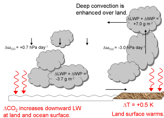
Figure 6: Conceptual picture of rapid tropical cloud changes due to increasing CO 2 shown together with mean tropical SP-CAM changes.
