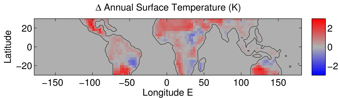
Figure 3: Annual mean change in surface temperature for SP-CAM due to 4xCO 2 .
