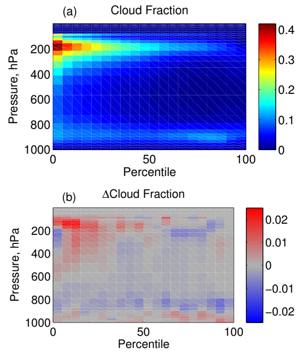
Figure 7: (a) \omega -sorted cloud fraction and (b) the change due to the \text{CO}_2 perturbation.
