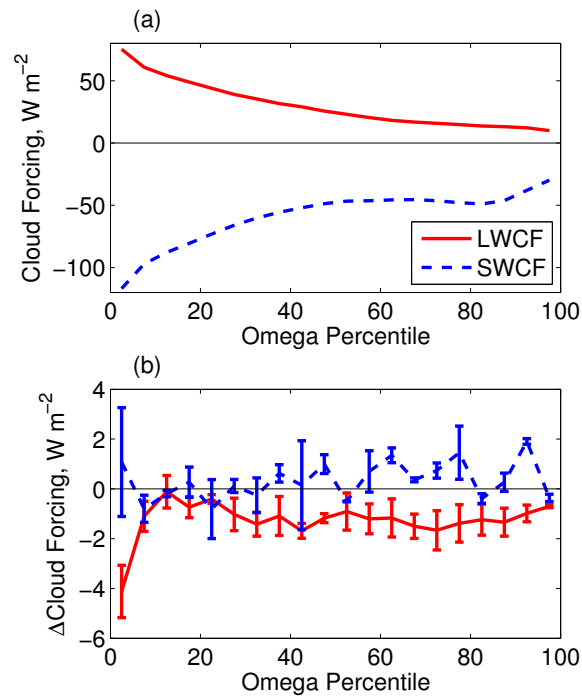
Figure 8: (a) SP-CAM \omega sorted longwave (red solid) and shortwave (blue dashed) cloud forcing in \text{W m}^{-2} and (b) changes in cloud forcing due to 4x\text{CO}_2 . Error bars are estimated from \omega changes in year 1 and year 2 computed separately.
