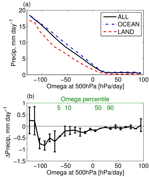
Figure 2: (a) Surface precipitation in mm day -1 for ocean (blue dot-dashed) land (red dashed), and tropics-wide (black solid) sorted by \omega_{500} . (b) Precipitation changes due to 4xCO 2 with error bars estimated from precipitation differences for simulation year 1 and year 2 considered separately. Omega percentiles are indicated in green at the top of the plot.
