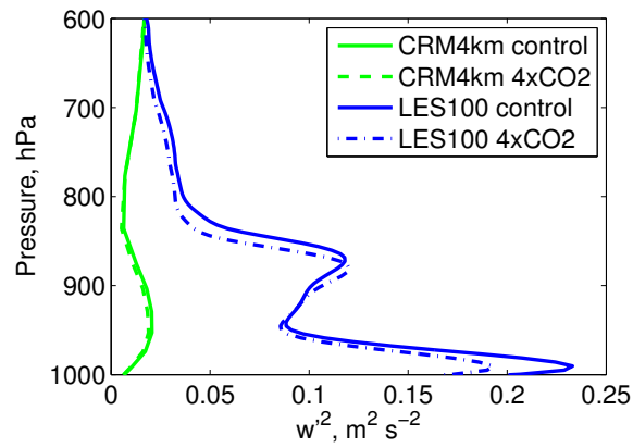
Figure 14: Vertical velocity variance \overline{w'^2} for LTS80-90 CRM4km and LES100 control and 4xCO 2 simulations in m 2 s -2 .
