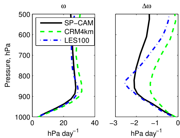
Figure 11: Pressure velocity \omega (left) and the difference in \omega for the 4xCO 2 case, \Delta\omega (right), for SP-CAM LTS 80-90th percentile, CRM4km, and LES100.
