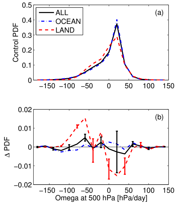
Figure 5: (a) PDF of tropical monthly pressure velocity \omega at 500 hPa and (b) its change due to 4xCO 2 , for SP-CAM. Separate PDF's are plotted for ocean (blue dash-dotted), land (red dashed) and all points (black solid). Error bars are estimated from PDF changes of years one and two considered separately.
