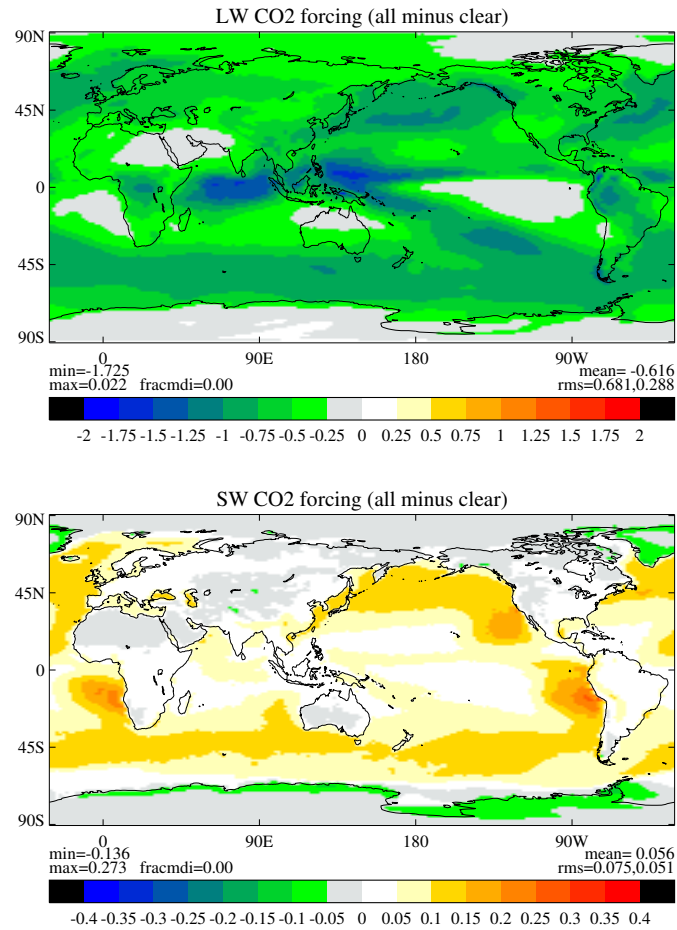
Figure 9: Change in calculated (a) LWCF and (b) SWCF in \text{W m}^{-2} due to instantaneous CO 2 doubling for HADGEM2 climate model, based on offline radiation calculations with clouds and other atmospheric and surface properties held fixed. Figure courtesy of Mark Webb, UK Met Office.
