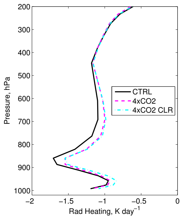
Figure 1: SP-CAM tropical mean heating rates in \text{K day}^{-1} for control (black solid), 4xCO 2 (magenta dashed), and control plus clear sky change due to 4xCO 2 (light blue dot-dashed, computed offline).
