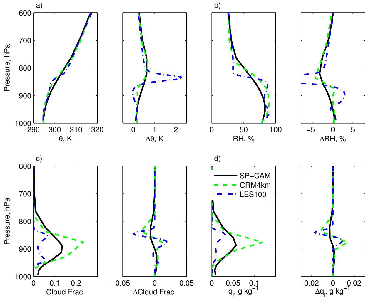
Figure 12: Comparison of SP-CAM, CRM4km, and LES100 profiles of a) potential temperature (K), b) relative humidity, c) cloud fraction, and d) cloud liquid water ( \text{g kg}^{-1} ) for the control (left) and the change with 4\times\text{CO}_2 (right). At the MBL inversion, the LES100 profile of \Delta RH in b) goes off the the displayed horizontal scale and extends to -27%.
