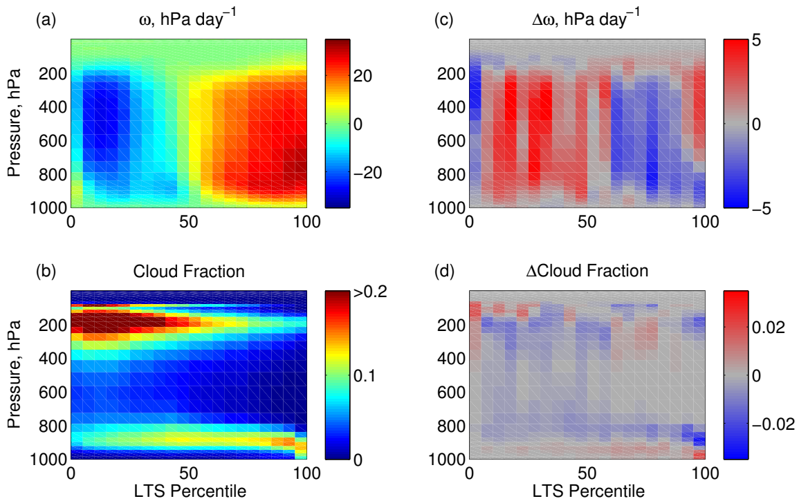
Figure 10: Monthly-mean tropical ocean profiles sorted by LTS for the SP-CAM. Control case (a) 500 hPa pressure velocity \omega and (b) cloud fraction, and corresponding 4xCO 2 changes, (c)-(d).
