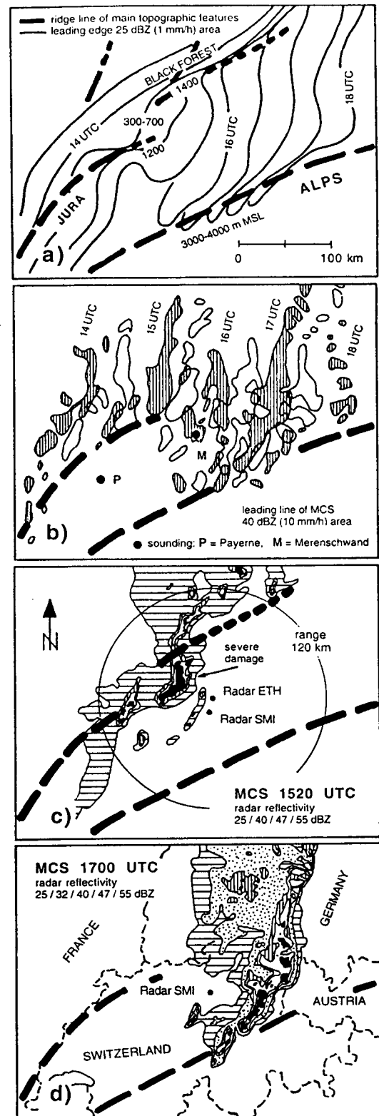
Figure 2. Development of MCS on 22 July 1995. a) movement of the leading edge (25 dBZ) and b) of the line of intense echo (40 dBZ), c) MCS at 1520 UTC (tornadic stage), d) MCS at 17 UTC (maximum organization).
