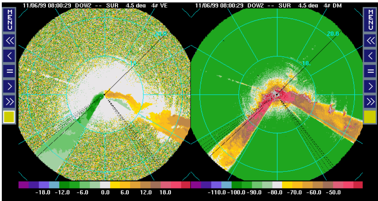
Figure 3. Low-elevation (4.5 deg) surveillance scan (PPI) collected at 08:00 UTC on November 6, 1999 in the Toce river valley. The DOW radar was located at the Pieve Vergonte site (center of the panels). The radial Doppler velocities are shown in the left panel and received power in the right panel. Range rings are indicated every 10 km. The topography restricted the radar observations at low levels to within the valley. Pieve Vergonte is located right at the bend of the Toce river valley. Down the valley is towards the bottom left ("220 deg") and up the valley is towards the right ("120 deg"). [Note: 1) North in the data ("0 deg") does not correspond to true north but rather where the DOW truck was pointing! True north is approximately in up-valley direction. 2) The received power indicated in the right panel is approximately 20 dB high compared to Figure 2 because of a removed signal attenuator without compensation.]
