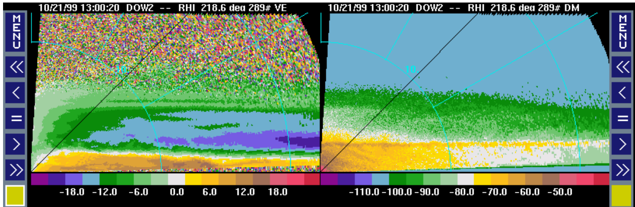
Figure 2. Vertical cross section (RHI) collected at 13:00 UTC on October 21, 1999 in the direction down the Toce river valley towards the Lago Maggiore. The DOW radar was located at the Pieve Vergonte site (left corner in the panels). The radial Doppler velocities are shown in the left panel and received power in the right panel. Range rings are indicated every 10 km.
