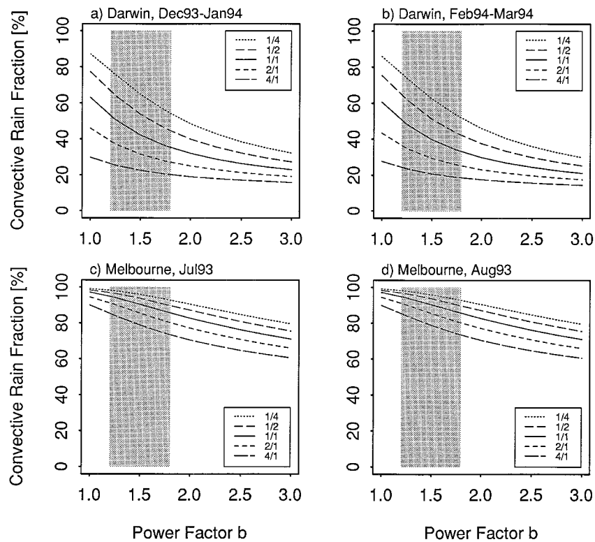
FIG. 2. Same as Fig. 1 except for data collected during four different time periods at two sites. (a) Darwin, December 1993–January 1994; (b) Darwin, February 1994–March 1994; (c) Melbourne, July 1993; and (d) Melbourne, August 1993.
