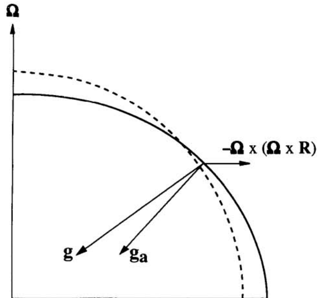
FIG. 1. Deformation of the earth's surface from a true sphere (dashed line) to an oblate spheroid (solid line). True gravity, indicated by the vector g , is perpendicular to the spherical surface. Apparent gravity g_a , being the vector sum of g and the centrifugal force -\boldsymbol{\Omega} \times (\boldsymbol{\Omega} \times \mathbf{R}) , is perpendicular to the surface of the oblate spheroid.
