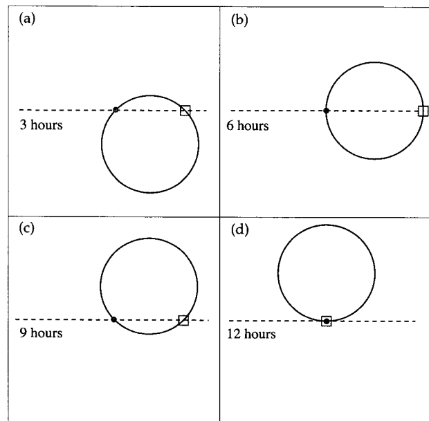
FIG. 3. Relative position of the fixed- and rotating-coordinate trajectories shown in Fig. 2 at 3, 6, 9, and 12 h. As in Fig. 2 the position of the air parcel is indicated by the open square. The North Pole is indicated by the heavy dot. The inertia circle trajectory rotates with the earth, turning 180^\circ around the pole in 12 h.
