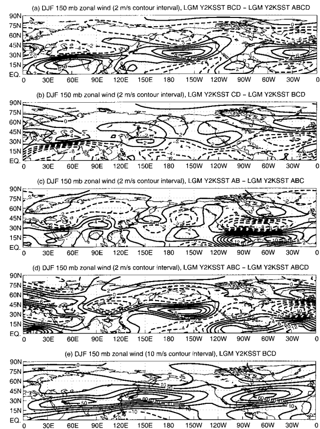
FIG. A8. Difference in DJF 150-mb zonal wind between these four pairs of CCM3 experiments: (a) LGM Y2KSST BCD - LGM Y2KSST ABCD, (b) LGM Y2KSST CD - LGM Y2KSST BCD, (c) LGM Y2KSST AB - LGM Y2KSST ABC, and (d) LGM Y2KSST ABC - LGM Y2KSST ABCD. (e) The total DJF zonal wind field for CCM3 experiment LGM Y2KSST BCD is shown. The contour interval for (a)–(d) is 2 \text{ m s}^{-1} , and the contour interval for panel (e) is 10 \text{ m s}^{-1} with dashed lines indicating negative contours.
