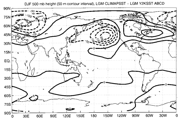
FIG. A2. Difference in DJF 500-mb geopotential height between CCM3 experiments LGM CLIMAPSST and LGM Y2KSST ABCD. The contour interval is 50 m with dashed lines indicating negative contours.
