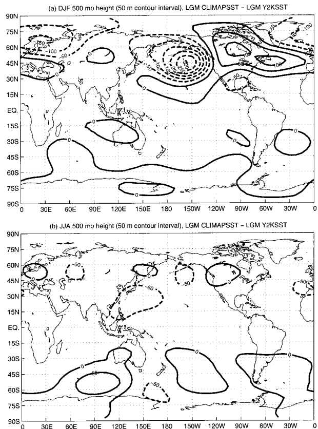
FIG. 10. As in Fig. 3, but for the difference in 500-mb geopotential height between CCM3 experiments LGM CLIMAPSST and LGM Y2KSST.
