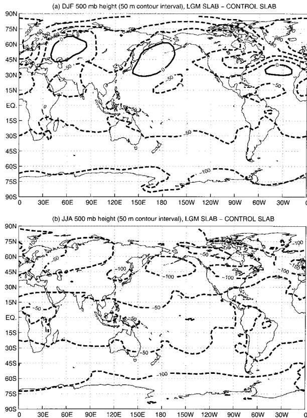
FIG. 5. As in Fig. 3, but for the difference in 500-mb geopotential height between CCM3 experiments LGM SLAB and CONTROL SLAB.
