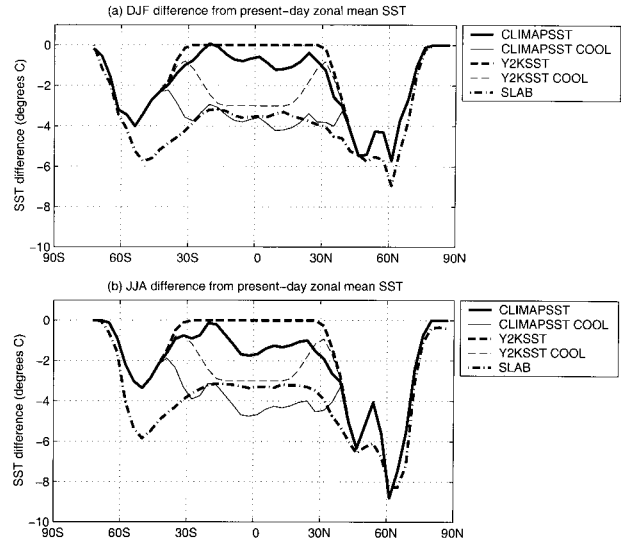
FIG. 2. The zonally averaged difference between present-day SST and the prescribed SST in experiments LGM CLIMAPSST (thick solid line), LGM CLIMAPSST COOL (thin solid line), LGM Y2KSST (thick dashed line), and LGM Y2KSST COOL (thin dashed line) in two seasons: (a) DJF and (b) JJA. The thick dashed-dotted line shows the zonally averaged difference in calculated SST between experiments LGM SLAB and CONTROL SLAB.
