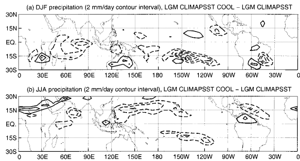
FIG. 13. As in Fig. 4, but for the difference in precipitation between CCM3 experiments LGM CLIMAPSST COOL and LGM CLIMAPSST.
