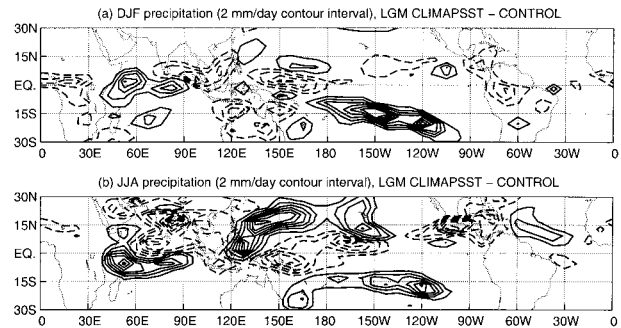
FIG. 4. Difference in precipitation between CCM3 experiments LGM CLIMAPSST and CONTROL in two seasons: (a) DJF and (b) JJA. The contour interval is 2 mm day -1 with dashed lines indicating negative contours and the zero contour omitted.
