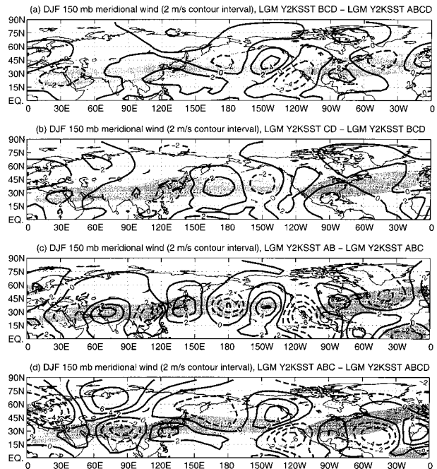
FIG. A10. Difference in DJF 150-mb meridional wind between these four pairs of CCM3 experiments: (a) LGM Y2KSST BCD – LGM Y2KSST ABCD, (b) LGM Y2KSST CD – LGM Y2KSST BCD, (c) LGM Y2KSST AB – LGM Y2KSST ABC, and (d) LGM Y2KSST ABC – LGM Y2KSST ABCD. The contour interval for (a)–(d) is 2 \text{ m s}^{-1} with dashed lines indicating negative contours. Regions where the DJF 150-mb wind exceeds 30 \text{ m s}^{-1} in the first of the two experiments differenced in each are shaded to indicate the locations of the jets.
