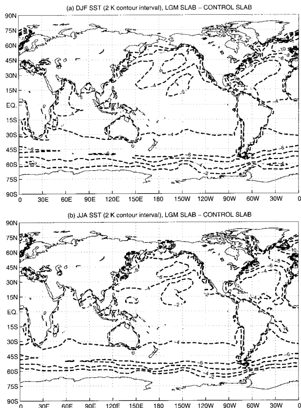
FIG. 7. Difference in SST between CCM3 experiments LGM SLAB and CONTROL SLAB in two seasons: (a) DJF and (b) JJA. The contour interval is 2^{\circ} C with dashed lines indicating negative contours.
