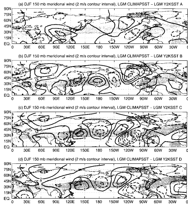
FIG. A9. Difference in DJF 150-mb meridional wind between CCM3 experiments LGM CLIMAPSST and these four experiments: (a) LGM Y2KSST A, (b) LGM Y2KSST B, (c) LGM Y2KSST C, and (d) LGM Y2KSST D. The contour interval for (a)–(d) is 2 \text{ m s}^{-1} with dashed lines indicating negative contours. Regions where the DJF 150-mb zonal wind exceeds 30 \text{ m s}^{-1} in experiment LGM CLIMAPSST are shaded to indicate the locations of the jets.
