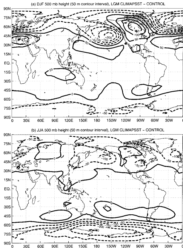
FIG. 3. Difference in 500-mb geopotential height between CCM3 experiments LGM CLIMAPSST and CONTROL in two seasons: (a) DJF and (b) JJA. The contour interval is 50 m with dashed lines indicating negative contours.
