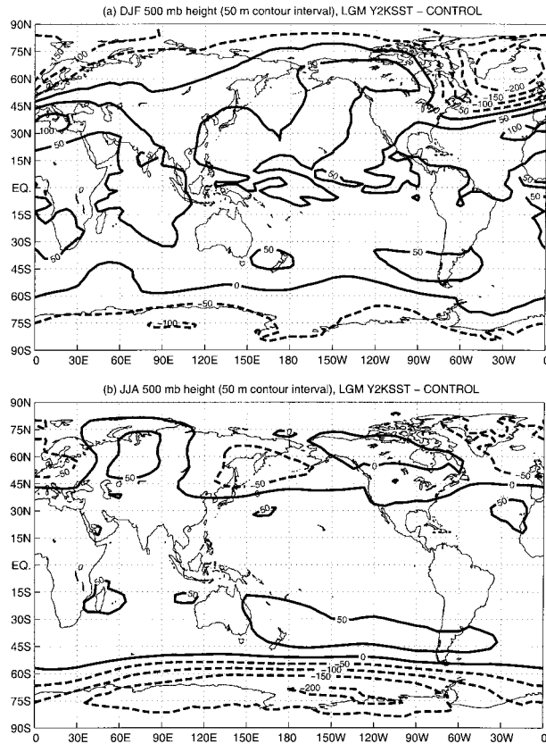
FIG. 8. As in Fig. 3, but for the difference in 500-mb geopotential height between CCM3 experiments LGM Y2KSST and CONTROL.
