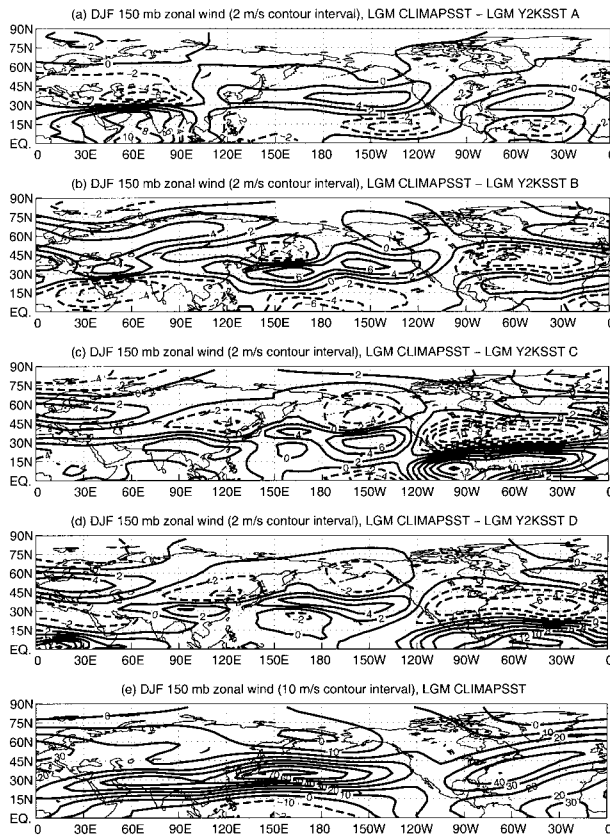
FIG. A7. Difference in DJF 150-mb zonal wind between CCM3 experiments LGM CLIMAPSST and these four experiments: (a) LGM Y2KSST A, (b) LGM Y2KSST B, (c) LGM Y2KSST C, and (d) LGM Y2KSST D. (e) The total DJF zonal wind field for CCM3 experiment LGM CLIMAPSST is shown. The contour interval for (a)–(d) is 2 \text{ m s}^{-1} , and the contour interval for (e) is 10 \text{ m s}^{-1} with dashed lines indicating negative contours.
