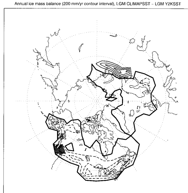
FIG. 12. The difference in annual mass balance (snowfall – melt) between CCM3 experiments LGM CLIMAPSST and LGM Y2KSST. The contour interval is 200\text{ mm yr}^{-1} (liquid water equivalent) with dashed lines indicating negative contours and the zero contour emphasized with a thick solid line.
