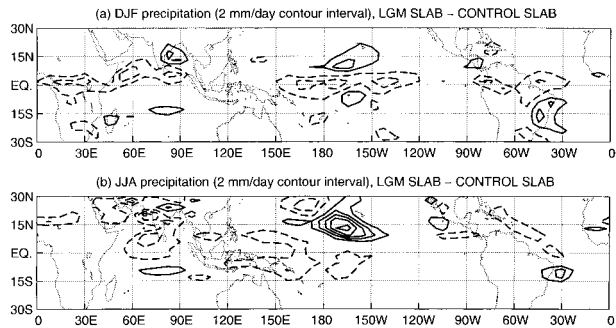
FIG. 6. As in Fig. 4, but for the difference in precipitation between CCM3 experiments LGM SLAB and CONTROL SLAB.
