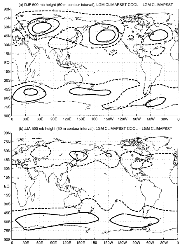
FIG. 14. As in Fig. 3, but for the difference in 500-mb geopotential height between CCM3 experiments LGM CLIMAPSST COOL and LGM CLIMAPSST.
