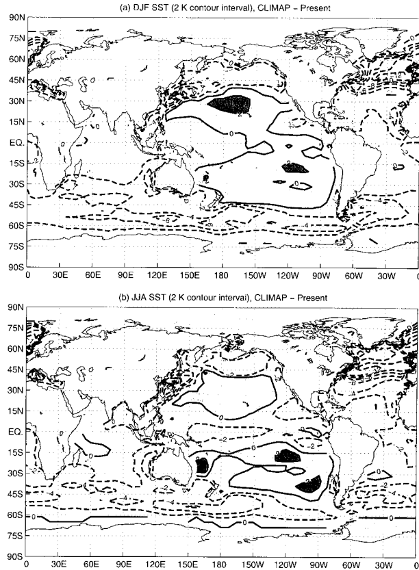
FIG. 1. The difference between the CLIMAP reconstruction of SST at the LGM and the present SST climatology in two seasons: (a) DJF and (b) JJA. The contour interval is 2°C, with dashed lines indicating negative contours. Regions of positive differences in SST are shaded.
