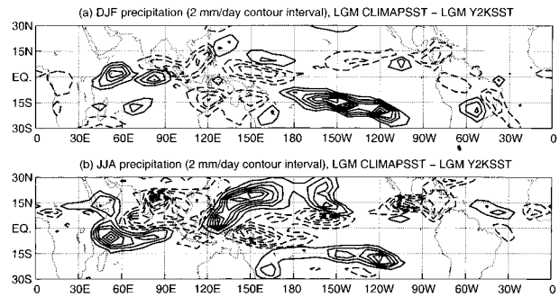
FIG. 9. As in Fig. 4, but for the difference in precipitation between CCM3 experiments LGM CLIMAPSST and LGM Y2KSST.
