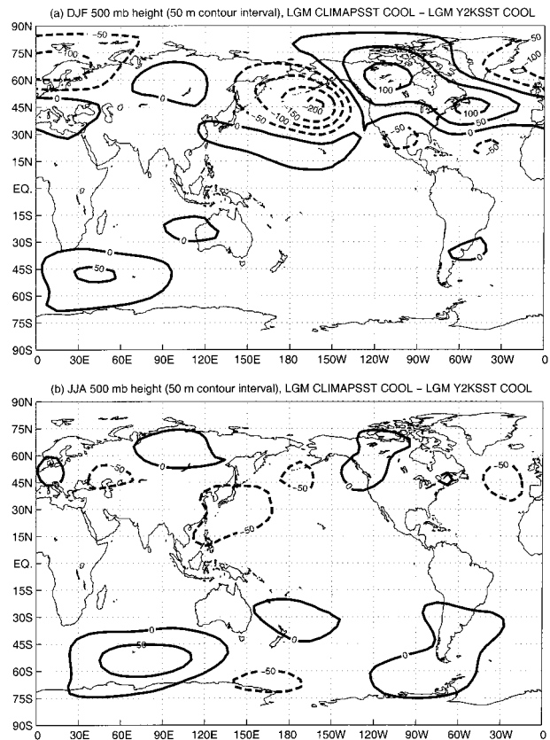
FIG. 15. As in Fig. 3, but for the difference in 500-mb geopotential height between CCM3 experiments LGM CLIMAPSST COOL and LGM Y2KSST COOL.
