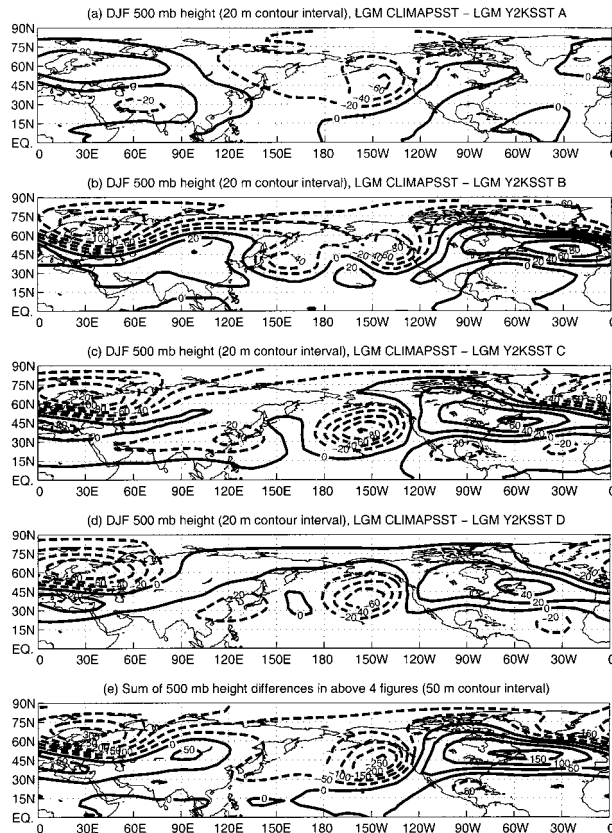
FIG. A3. Difference in DJF 500-mb geopotential height between CCM3 experiment LGM CLIMAPSST and these four experiments: (a) LGM Y2KSST A, (b) LGM Y2KSST B, (c) LGM Y2KSST C, and (d) LGM Y2KSST D. The sum of the differences in (a)–(d) is shown in (e). The contour interval for (a)–(d) is 20 m, and the contour interval for (e) is 50 m with dashed lines indicating negative contours.
