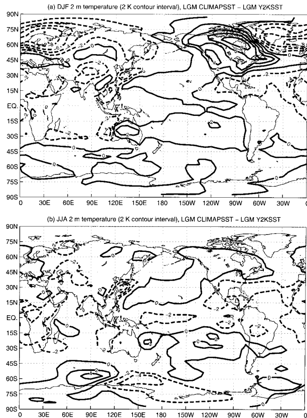
FIG. 11. Difference in reference height (2 m) temperature between CCM3 experiments LGM CLIMAPSST and LGM Y2KSST in two seasons: (a) DJF and (b) JJA. The contour interval is 2^{\circ}\text{C} , with dashed lines indicating negative contours.
