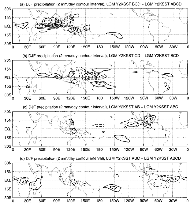
FIG. A6. Difference in DJF precipitation between these four pairs of CCM3 experiments: (a) LGM Y2KSST BCD – LGM Y2KSST ABCD, (b) LGM Y2KSST CD – LGM Y2KSST BCD, (c) LGM Y2KSST AB – LGM Y2KSST ABC, and (d) LGM Y2KSST ABC – LGM Y2KSST ABCD. The contour interval for (a)–(d) is 2 \text{ mm day}^{-1} with dashed lines indicating negative contours and the zero contour omitted.
