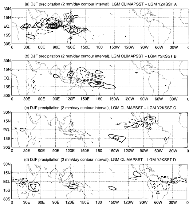
FIG. A5. Difference in DJF precipitation between CCM3 experiments LGM CLIMAPSST and these four experiments: (a) LGM Y2KSST A, (b) LGM Y2KSST B, (c) LGM Y2KSST C, and (d) LGM Y2KSST D. The contour interval for (a)–(d) is 2 \text{ mm day}^{-1} with dashed lines indicating negative contours and the zero contour omitted.
