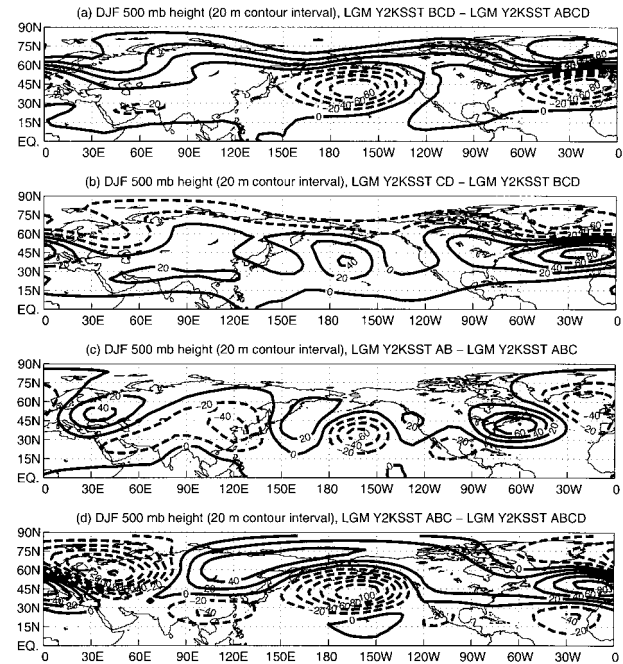
FIG. A4. Difference in DJF 500-mb geopotential height between these four pairs of CCM3 experiments: (a) LGM Y2KSST BCD - LGM Y2KSST ABCD, (b) LGM Y2KSST CD - LGM Y2KSST BCD, (c) LGM Y2KSST AB - LGM Y2KSST ABC, and (d) LGM Y2KSST ABC - LGM Y2KSST ABCD. The contour interval for (a)–(d) is 20 m with dashed lines indicating negative contours.
