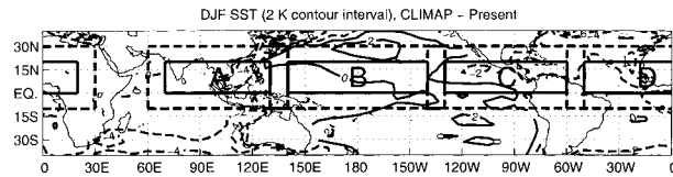
FIG. A1. The difference between the CLIMAP reconstruction of SST at the LGM and the present SST climatology in the Tropics during DJF. The contour interval is 2^{\circ}\text{C} with dashed lines indicating negative contours. Regions of positive differences in SST are shaded. The superimposed bold rectangles indicate regions A, B, C, and D of the CLIMAP tropical SST anomalies described in the text. The solid rectangles indicate the boundaries of the regions within which SSTs equal their present-day values, while the dashed rectangles indicate the boundaries of the regions outside of which SSTs equal their CLIMAP values. SSTs are linearly blended between CLIMAP and present-day values in the 10 degrees of lat and long between these rectangles.
