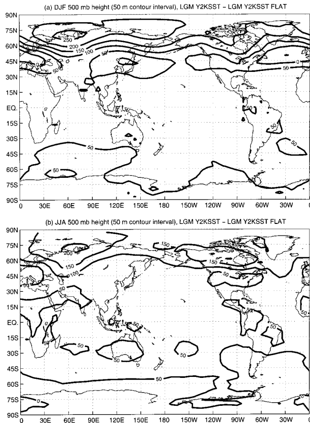
FIG. 16. As in Fig. 3, but for the difference in 500-mb geopotential height between CCM3 experiments LGM Y2KSST and LGM Y2KSST FLAT.
