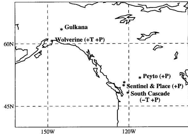
FIG. 1. Glacier locations are indicated by asterisks. Local wintertime climate variables that are found to be significantly correlated with anomalies in the net annual mass balance (NAB; section 3a) are indicated by P (precipitation) and T (temperature). Plus and minus signs indicate the sign of the correlation between climate variables and NAB.
