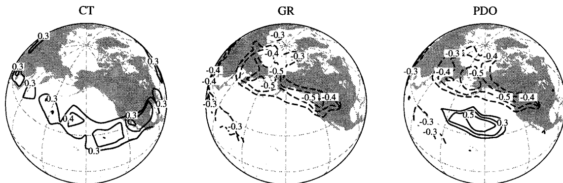
FIG. 11. Correlation maps of winter (NDJFMA) mean storminess with winter mean climate indexes for the period of record 1947–94. Contours show correlations that exceed the 95% confidence level where each year is considered to be independent of the last. Positive correlations indicate more storminess associated with warmer water in the tropical Pacific and colder water in the North Pacific.
