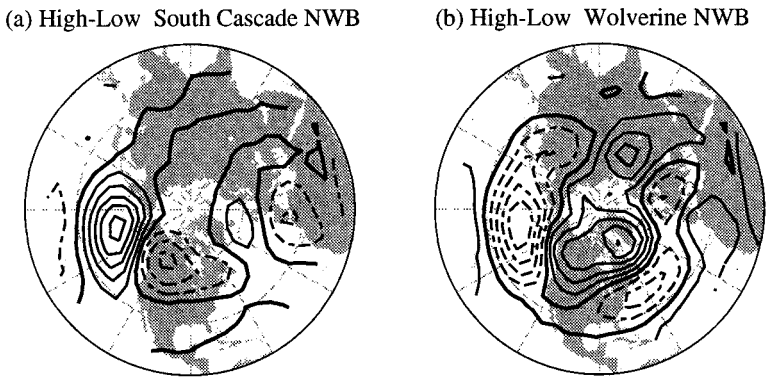
FIG. 8. Difference between composites from Fig. 7. The contour interval is 20 m.
