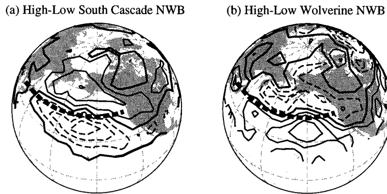
FIG. 9. Composite difference in storminess (defined as the rms of high-passed Z_{500} anomalies) for the high minus low years for the South Cascade and Wolverine glaciers. Climatological wintertime jet (maximum storminess in meridional direction) is shown by heavy dashed line. The contour interval is 3 m.
