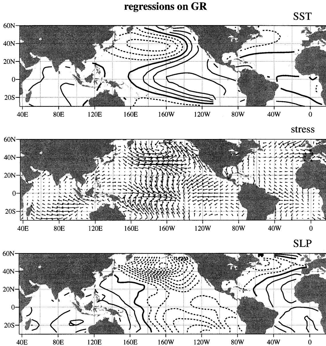
FIG. 4. Global fields regressed upon the monthly GR time series, displayed in Fig. 3: (a) SST, (b) wind stress, and (c) SLP. The contour interval is per unit standard deviation: (a) 0.1 K, (b) 8.3 \text{ m}^2 \text{ s}^{-1} for the longest vector, and (c) 0.1 mb. Negative contours are dashed and the zero contour is thickened. Reproduced from Fig. 11 of Zhang et al. (1997).
