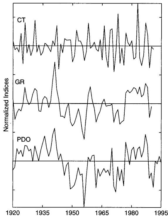
FIG. 3. Winter averaged values of the SST indexes. The plotting convention is such that, e.g., a datum plotted as 1954 is an average from Nov 1953 through Apr 1954.
