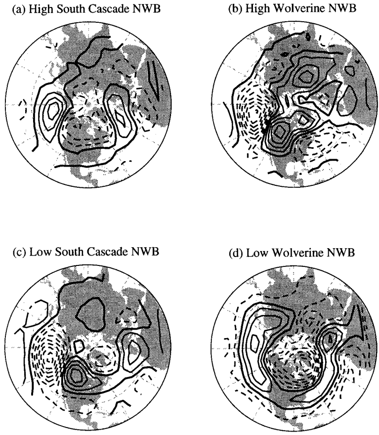
FIG. 7. As in Fig. 6, but the composites are 500-mb height anomalies, where anomalies are defined as departures from the climatological mean. The contour interval is 10 m.
