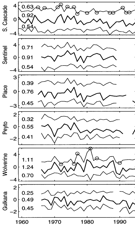
FIG. 2. Mass balance for the six glaciers used in this study: South Cascade, Sentinel, Place, Peyto, Wolverine, and Gulkana. In each panel, the NAB, \approx net annual accumulation minus net annual ablation, is the heavy solid line. The thin solid lines that bracket each NAB curve denote the net mass balance change over the winter (NWB, upper line) and summer (NSB, lower line) seasons. The data are aligned along the abscissa such that, e.g., NAB (1980) = NWB (1980) + NSB (1980), where NWB (1980) spans the period fall 1979–spring 1980, NSB (1980) spans late spring and summer of 1980, and NAB (1980) spans fall 1979 to the end of summer 1980. Standard deviations of each time series are shown on the left side of the curve. Units are in meters of liquid water equivalent. Breaks in the curve indicate missing data. For the South Cascade and Wolverine glaciers, anomalies in NWB greater than one standard deviation above and below the mean are denoted with circles (see section 3b).
