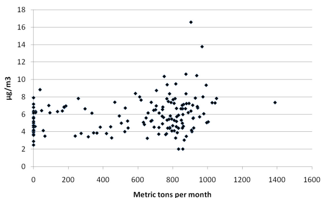
Fig. 3. Monthly mean fine mass concentration ( \text{PM}_{2.5} ) measured at Wishram vs PGE Boardman \text{NO}_x emissions (metric tons/month) for the period 1993–2006.
