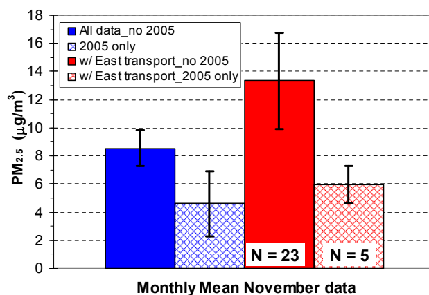
Fig. 4. Comparison of IMPROVE data from Wishram for all November data except 2005 (solid bars) with November 2005 data (cross-hatched). The comparison on the left (blue) is for all November data. The comparison on the right only includes those days with trajectories coming from the east end of the CRG. More detailed data are shown in Table 5, including 95% confidence intervals on each value.
