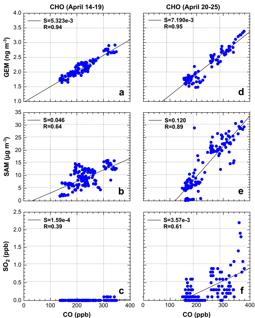
Fig. 3. Correlations in (a) CO and GEM, (b) CO and SAM, (c) CO and SO 2 for the period April 14–19, 2004; (d) CO and GEM, and (e) CO and SAM, (f) CO and SO 2 for the period April 20–25, 2004. The slope and R are shown for each relationship.
