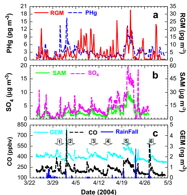
Fig. 2. Time series of (a) short-lived species RGM and PHg, (b) SO 4 and submicron aerosol mass (SAM), (c) GEM, CO and rainfall. The rainfall (arbitrary units) shown here is not from CHO but from the nearest two sites (Oku and Nago). The legends show the respective variables in each plate and the numbers in the lowest plate show the regional transport events.
