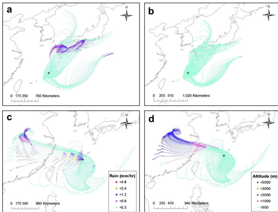
Fig. 4. NOAA-HYSPLIT 3 days back trajectories showing the history of rainfall and 3D movement of air masses for the two periods, April 14–19 (a, b, event #4) and April 20–25 (c, d event #5), respectively. For each event, we have calculated trajectories at 1-h intervals (120 trajectories). The rainfall and altitude of air parcels are shown by different colors. The arrival point of trajectories at CHO (26.8°N, 128.2°E, 60 m) is shown by the cross symbol.
